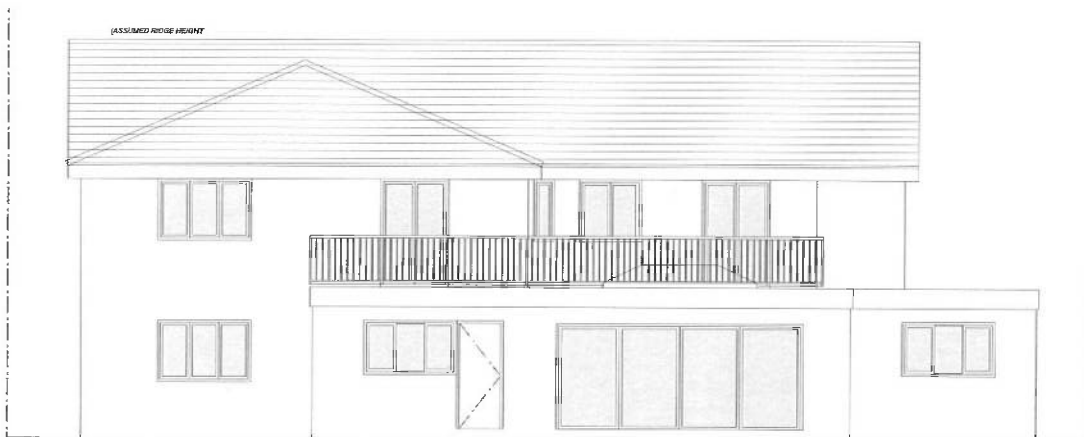
REAR ELEVATION (SOUTH FACADE)
