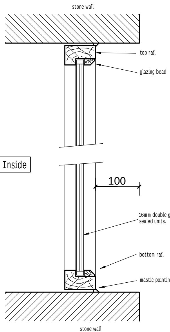
Vertical section 1 - 1 through fixed light (1:5)
