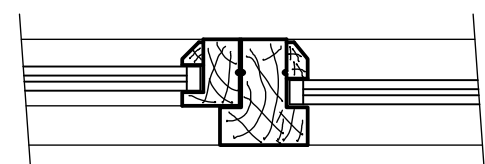
Horizontal section 5 - 5 through timber mullion (1:5)
