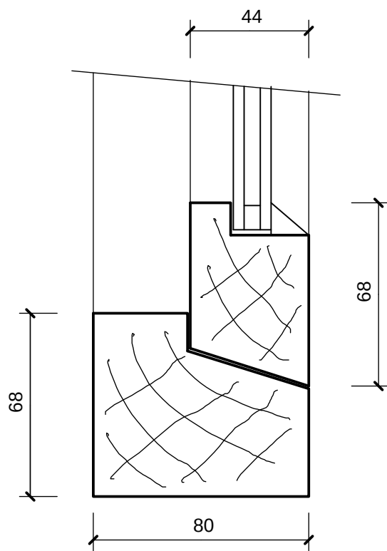
Section through window showing member sizes (1:2)
