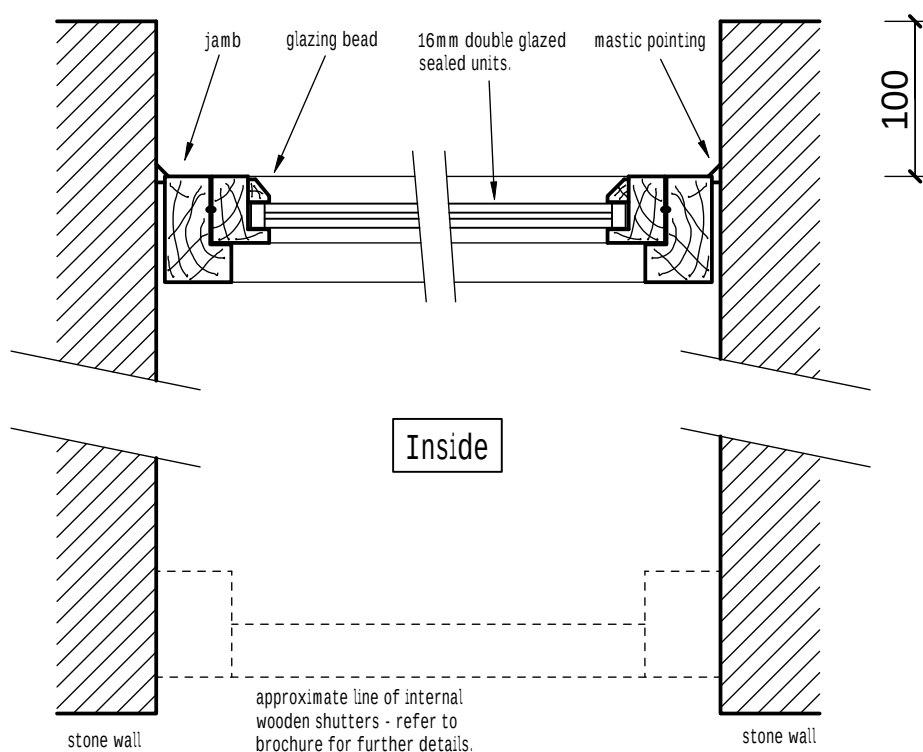
Horizontal section 4 - 4 through opening window (1:5)
