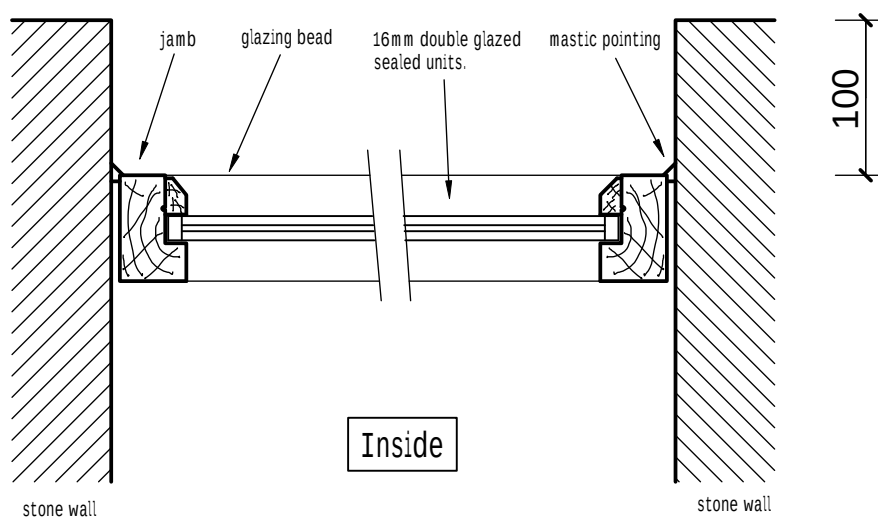
Horizontal section 3 - 3 through fixed light (1:5)
