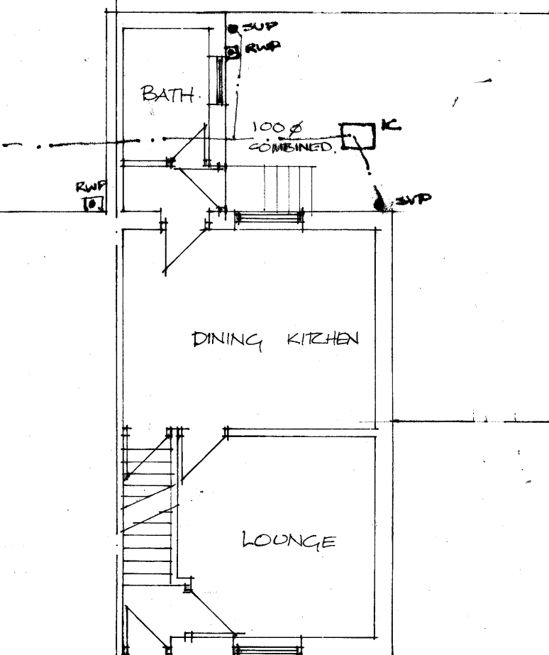
GROUND 1:100
