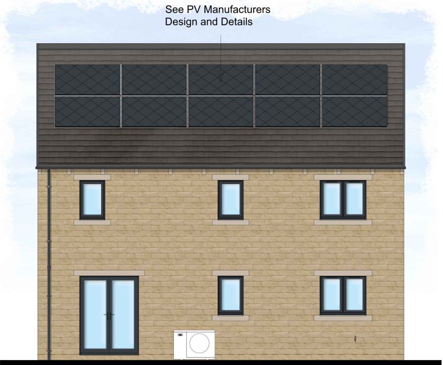
Rear Elevation
