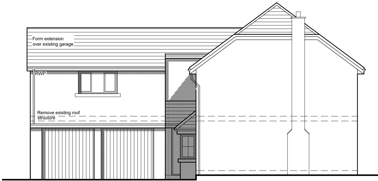
NORTH FACING ELEVATION
