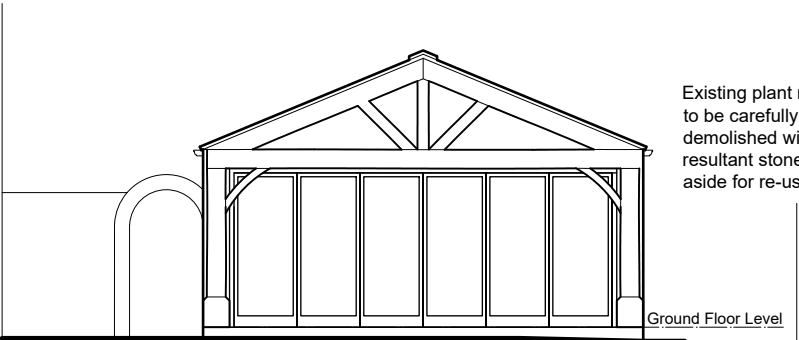
South Elevation (front)
