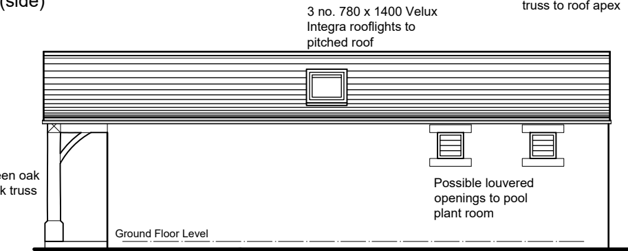
West Elevation (side)
