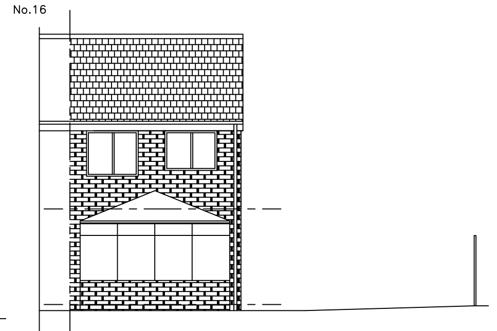
Existing Rear Elevation North-West
