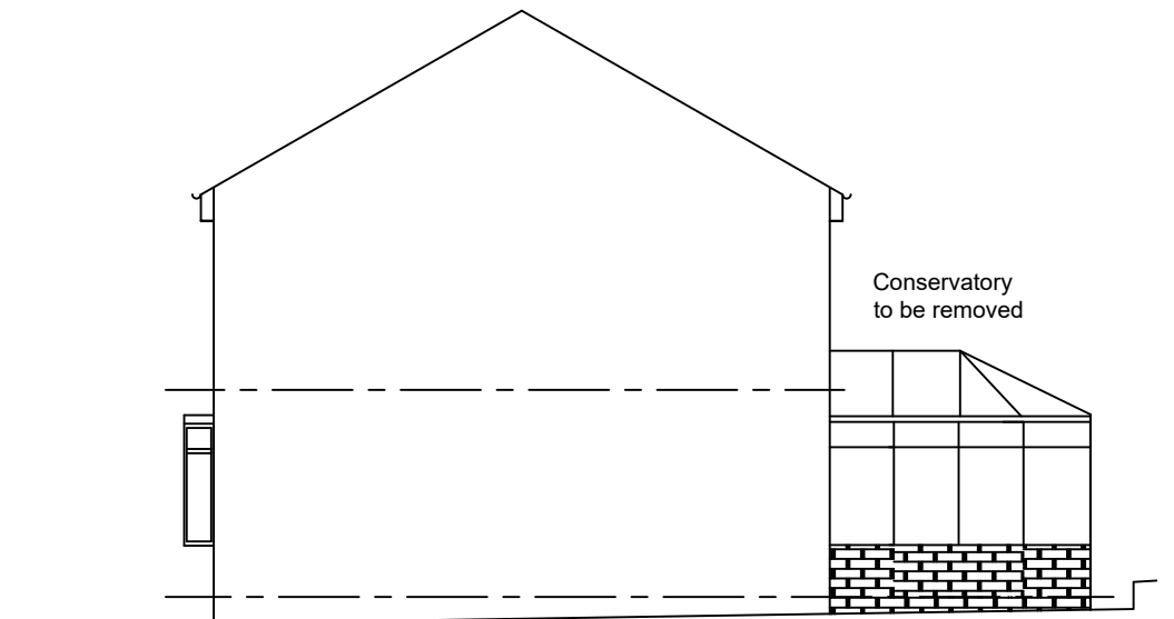
Existing Right Hand Side Elevation North East
