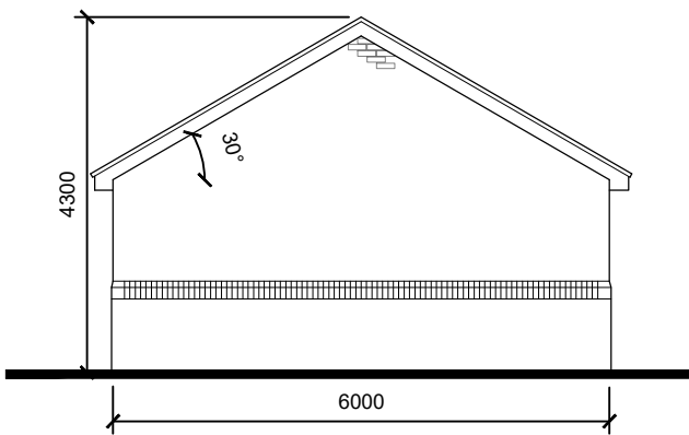
Rear Elevation
