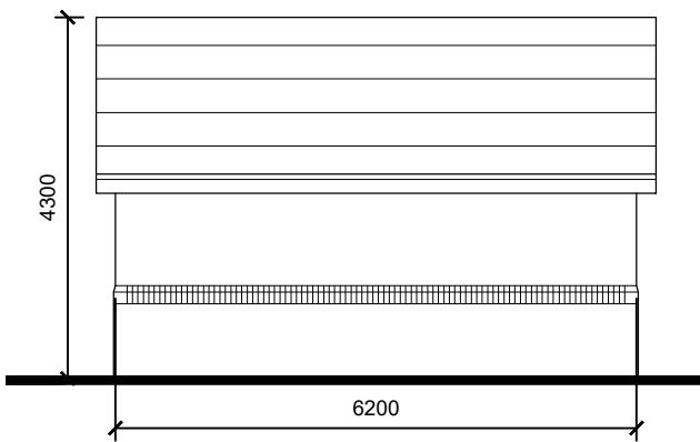
Side Elevations
