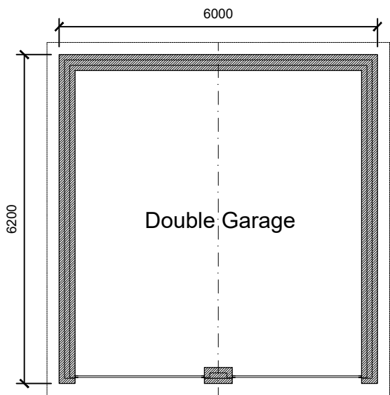
Garage Plan
