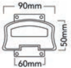
Top Bracket
