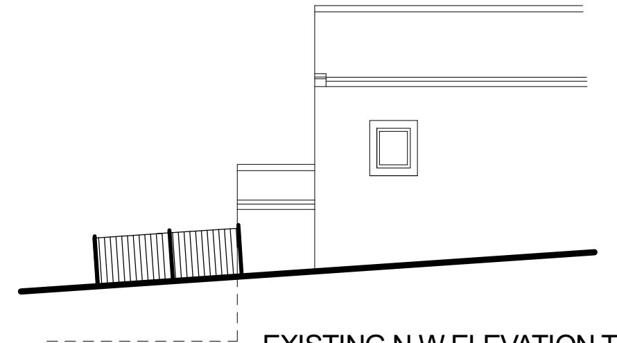
EXISTING N W ELEVATION TO UPPER WELLHOUSE ROAD
