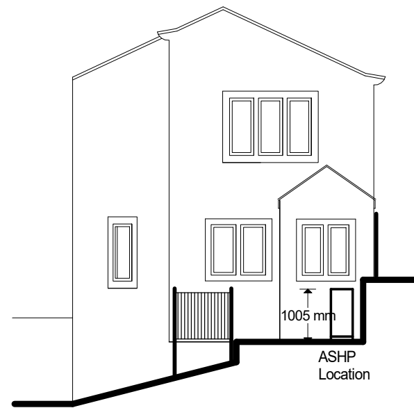
PROPOSED N E ELEVATION
