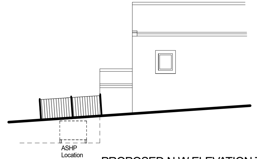
PROPOSED N W ELEVATION TO UPPER WELLHOUSE ROAD
