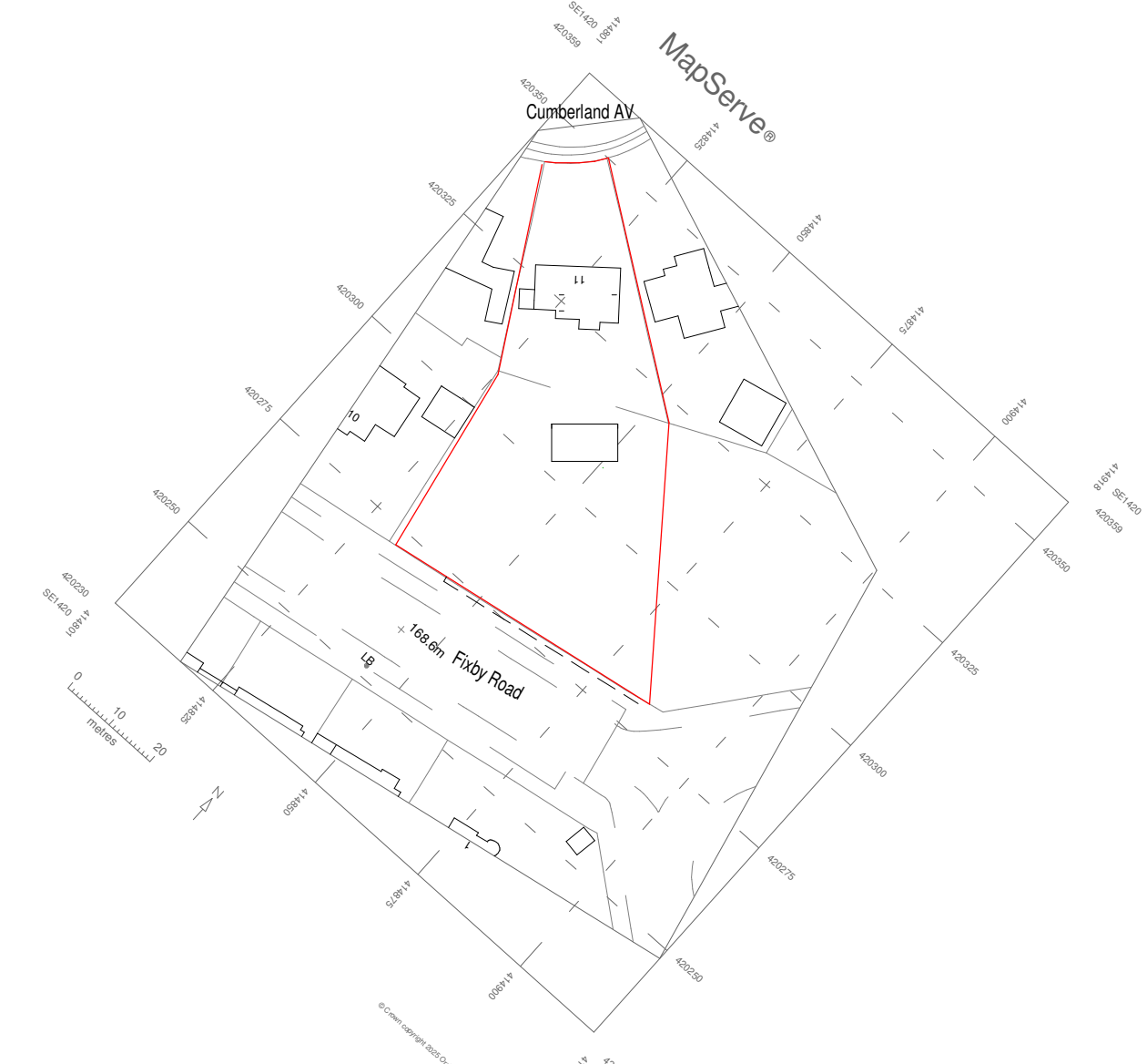
2 Location Plan 1 : 1250
