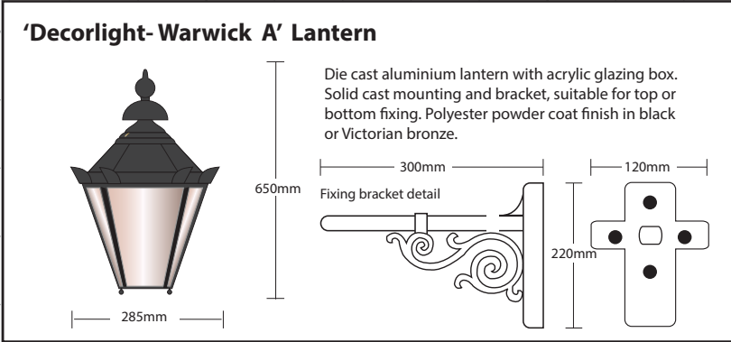
F FIVE X LANTERNS FINISHED BLACK. SIZE. 0.28m x 650mm. H.A.G. 2m.
