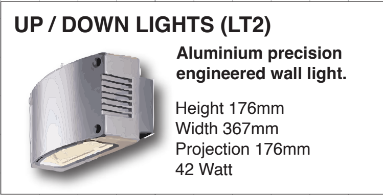
H FIVE X DOWN LIGHTS. SIZE. 0.36m x 176mm. H.A.G. 2.5m.
