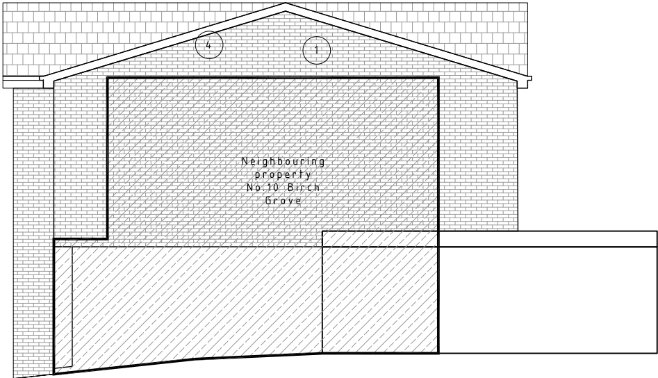
PROPOSED OTHER SIDE ELEVATION
