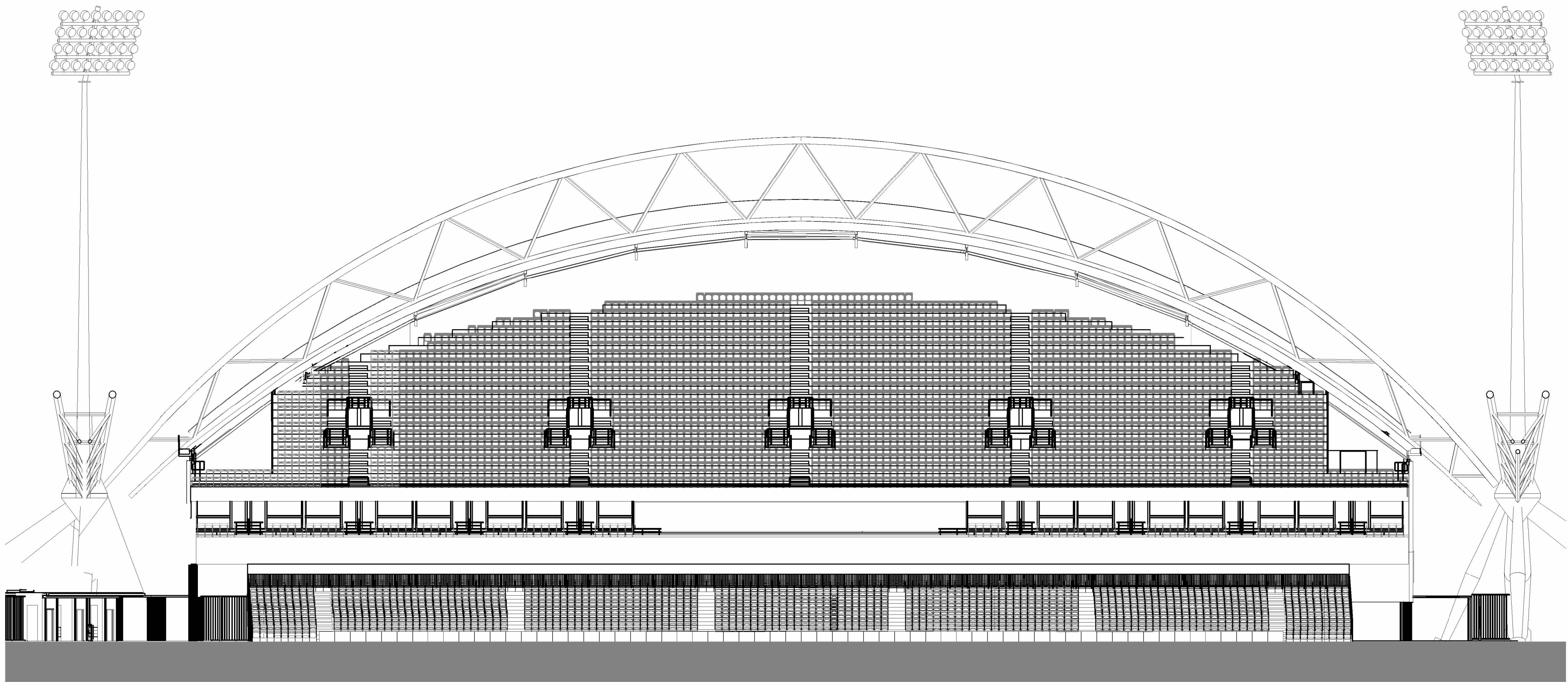
3 Existing South Western Elevation
