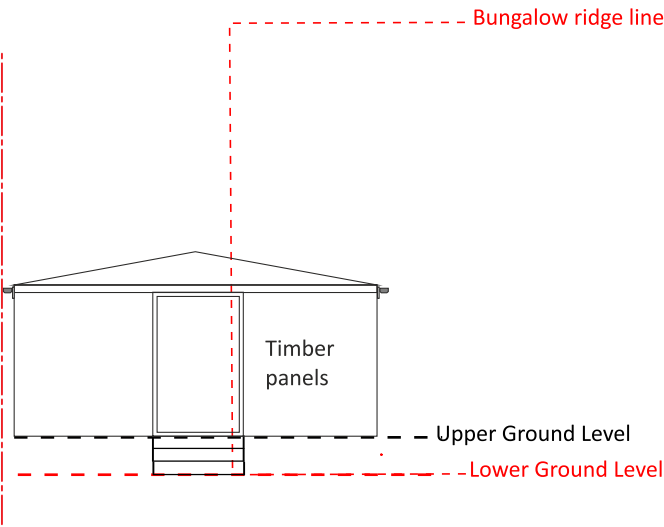
EXISTING EAST ELEVATION
