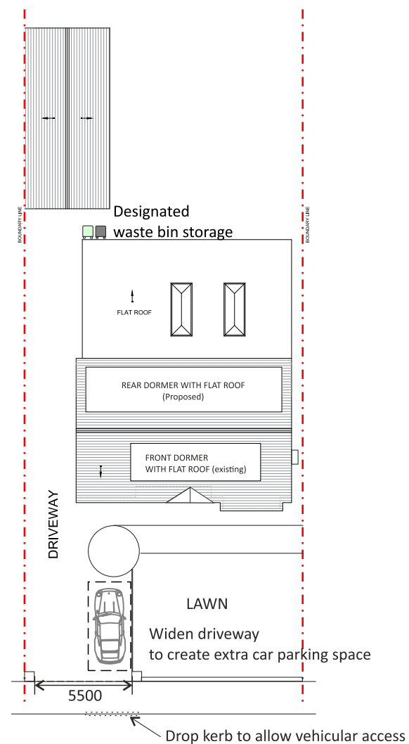
Proposed Parking Layout Scale 1:300
