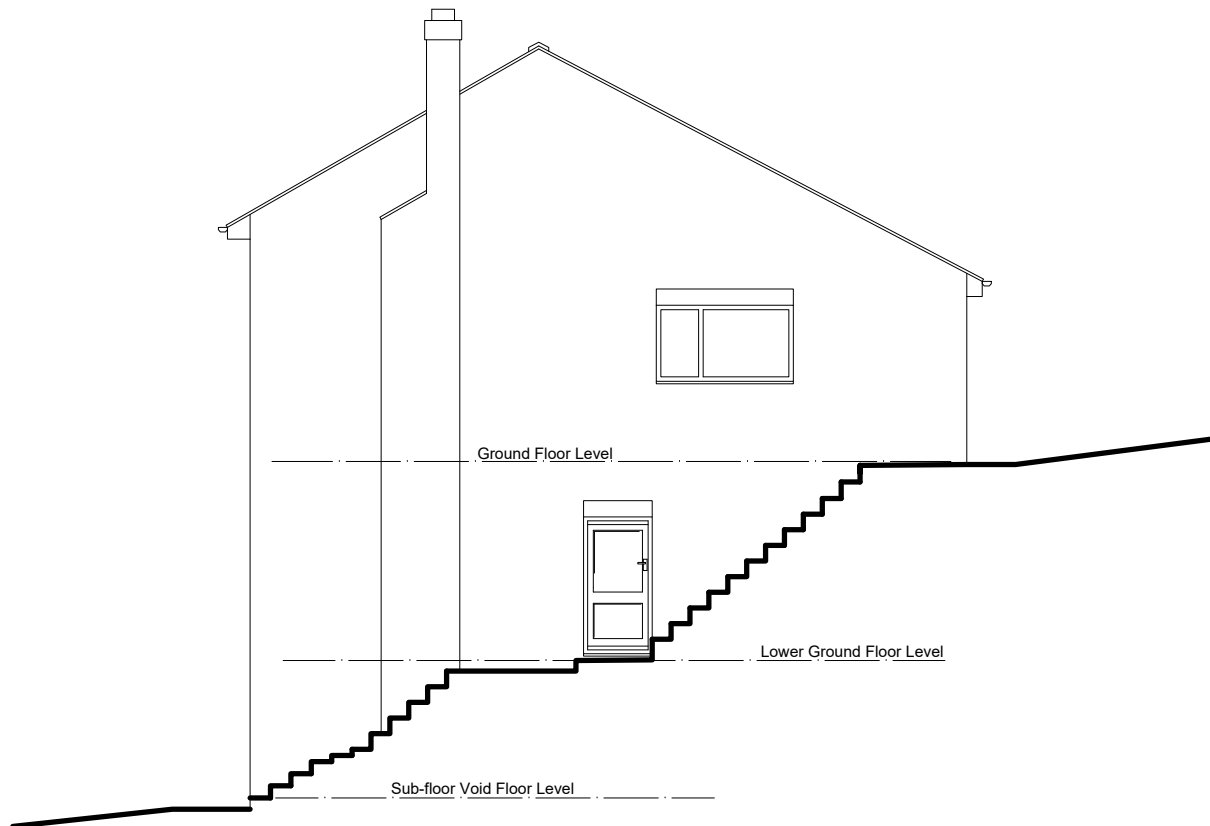
South West Elevation (side)
