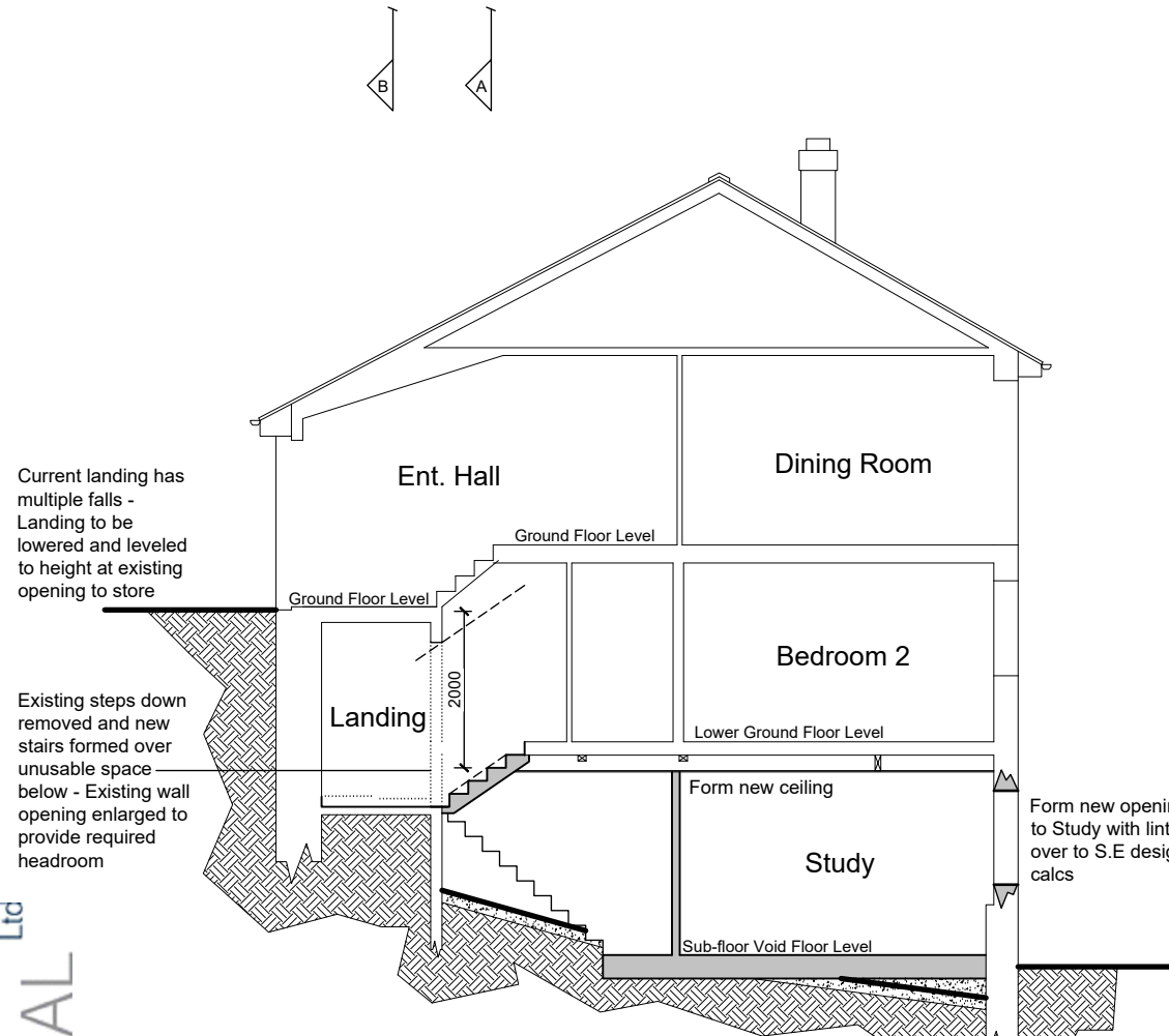
Section B-B
