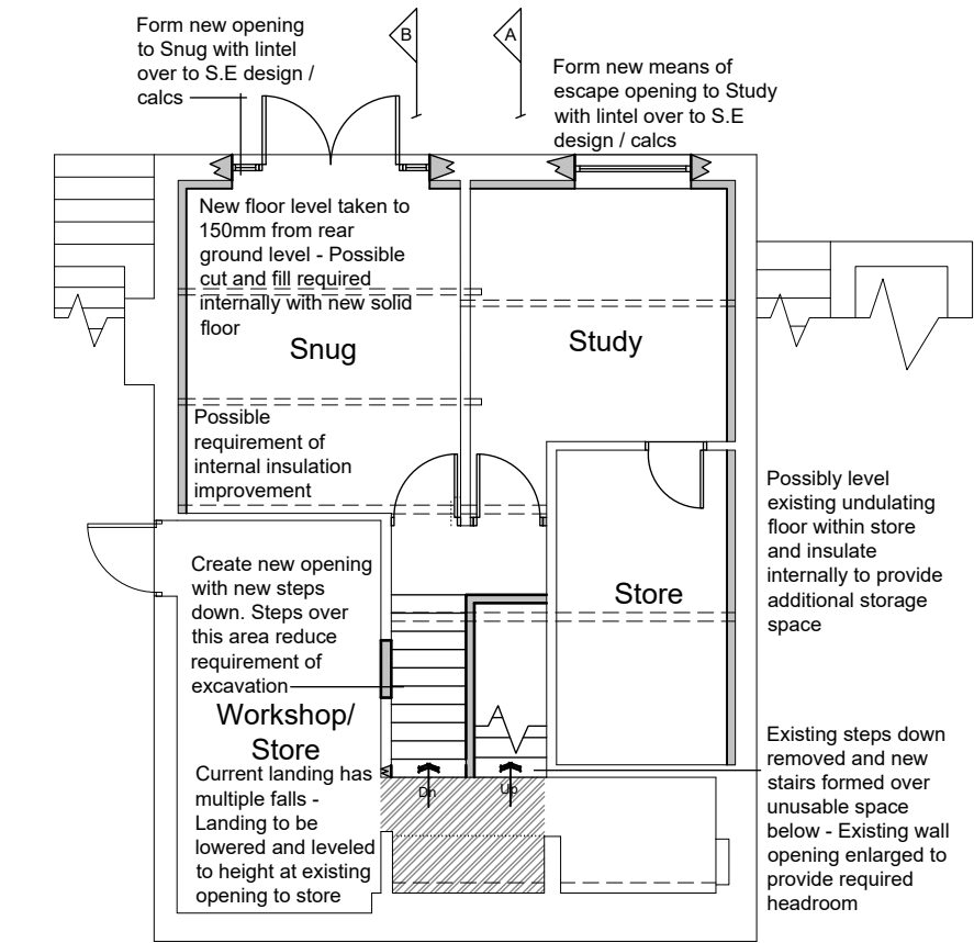
Sub-Floor Void Floor Plan
