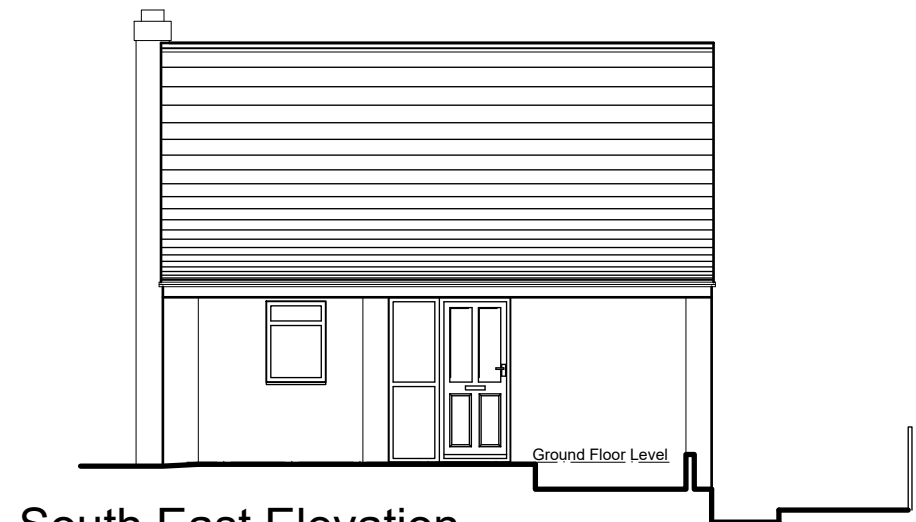
South East Elevation (front)
