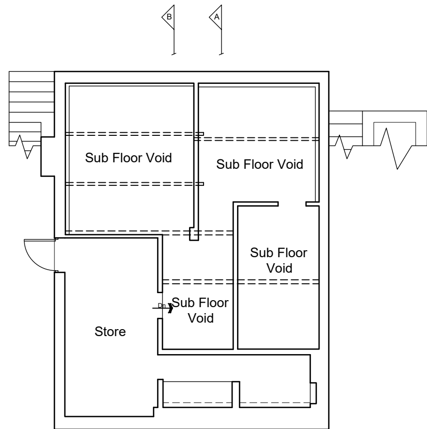
Sub-Floor Void Floor Plan
