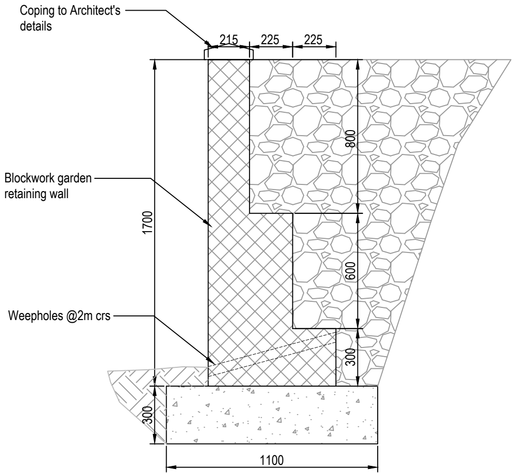
Section C-C Retaining Wall Type C (1:20)
