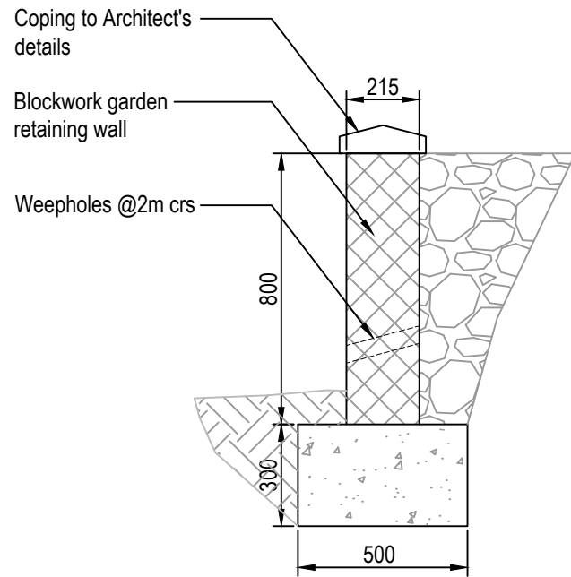
Section A-A Retaining Wall Type A (1:20)
