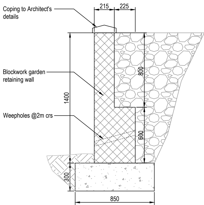
Section B-B Retaining Wall Type B (1:20)
