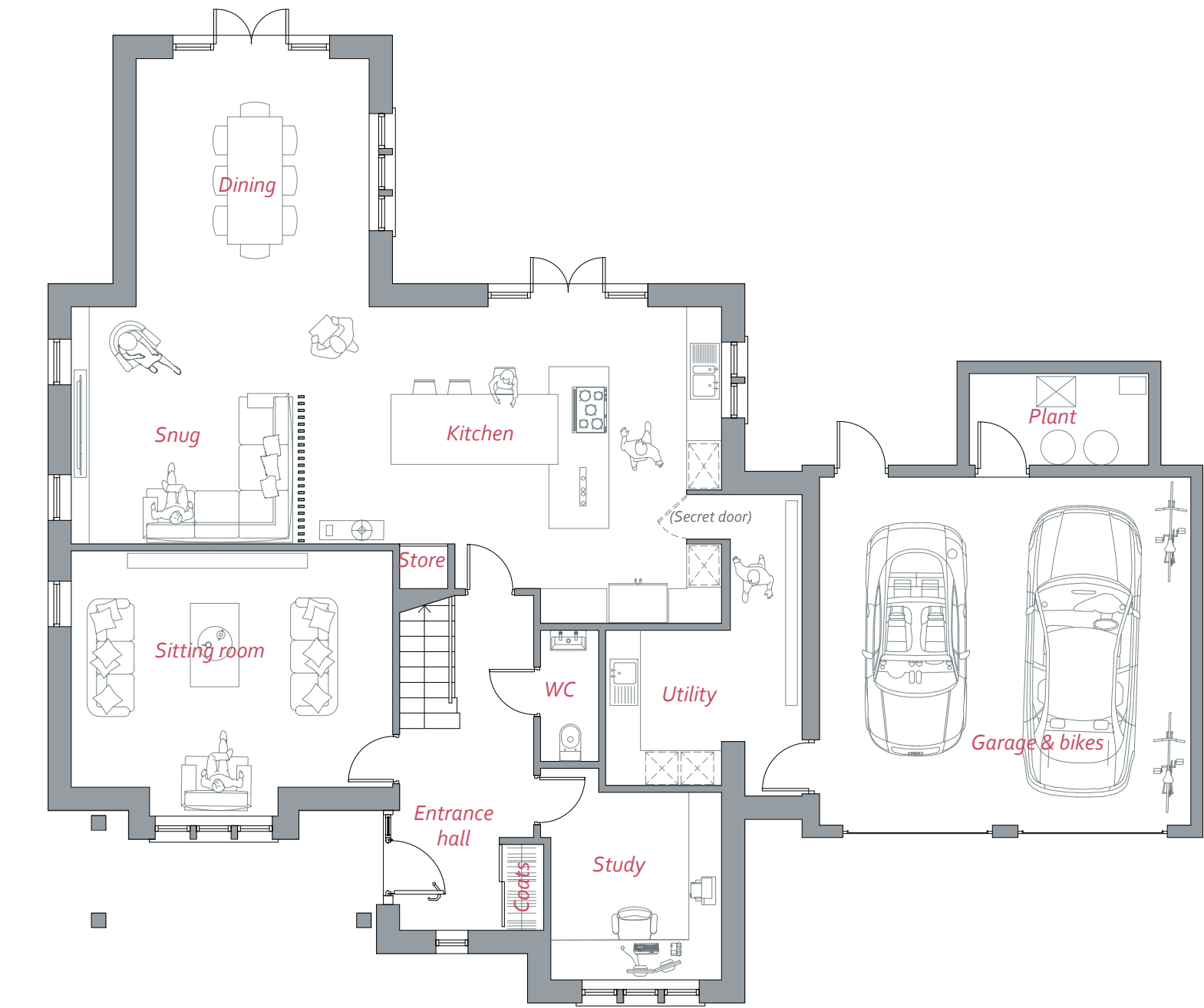
GROUND FLOOR
