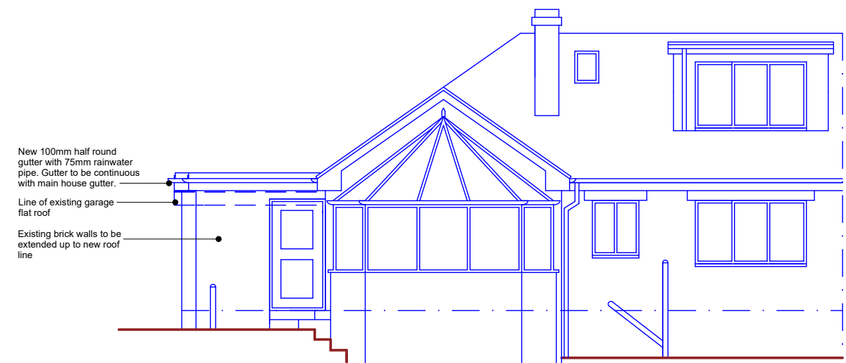
Rear Elevation (South)
