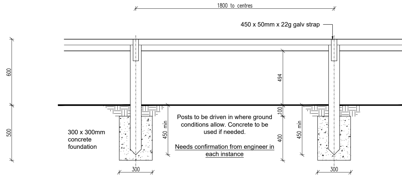
600mm Knee Rail
