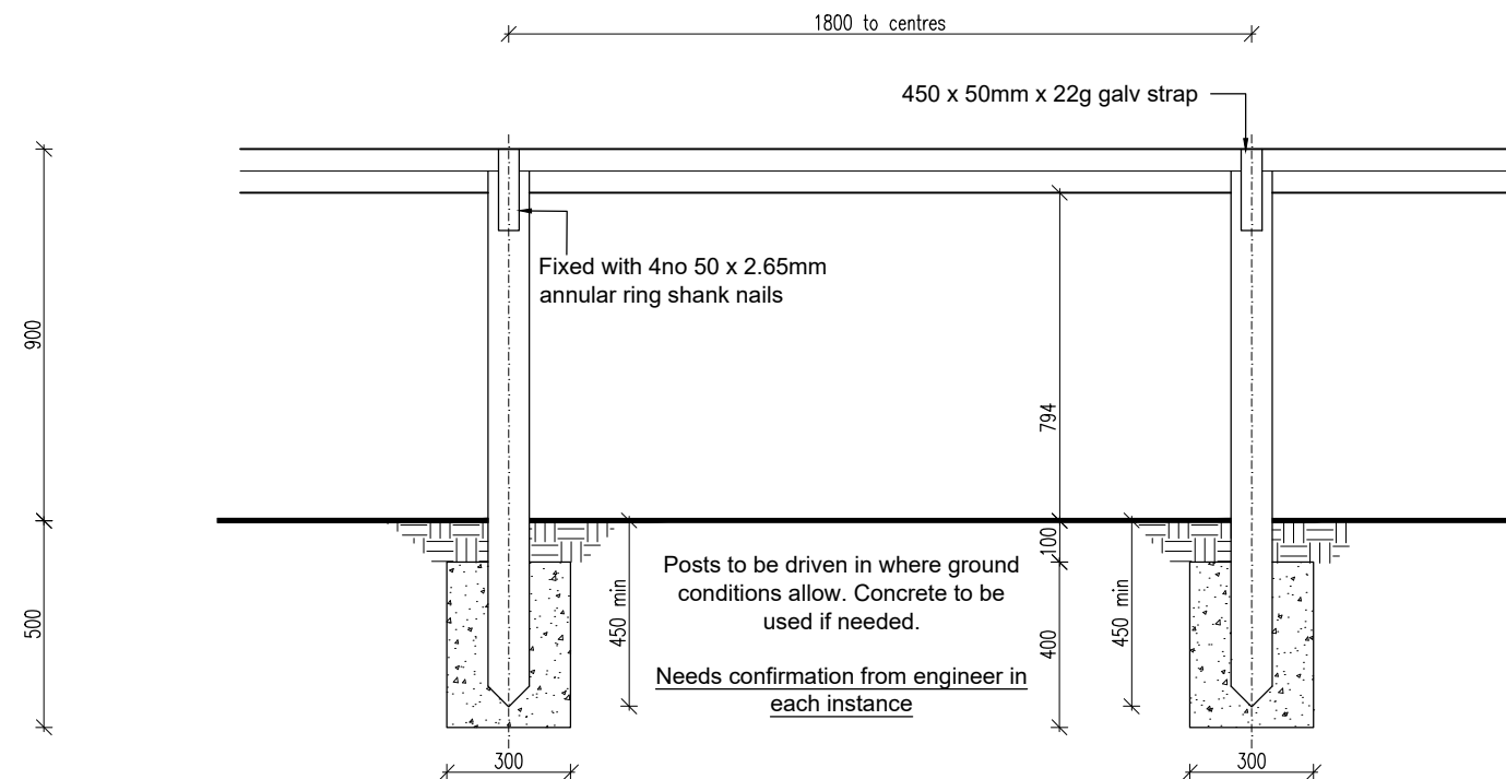
900mm Knee Rail
