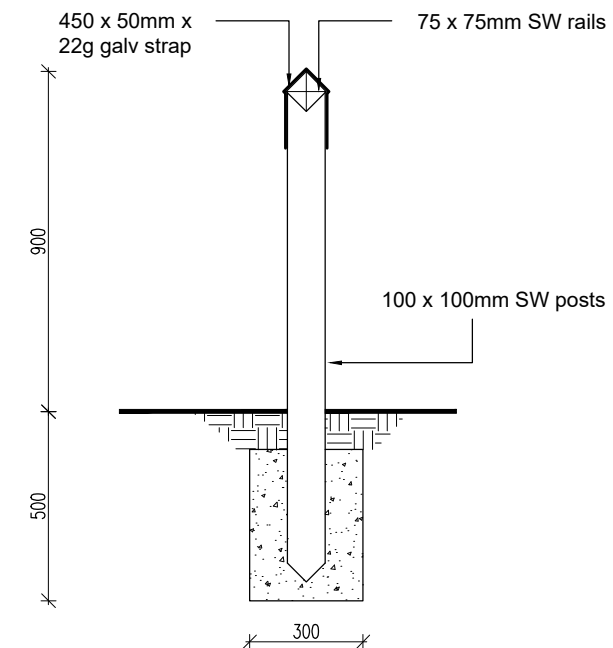
900mm - Section
