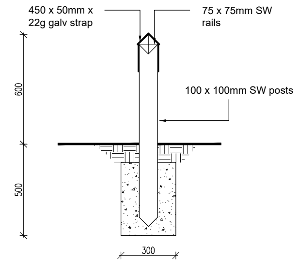
600mm - Section
