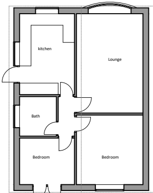
Existing Ground Floor Plan
