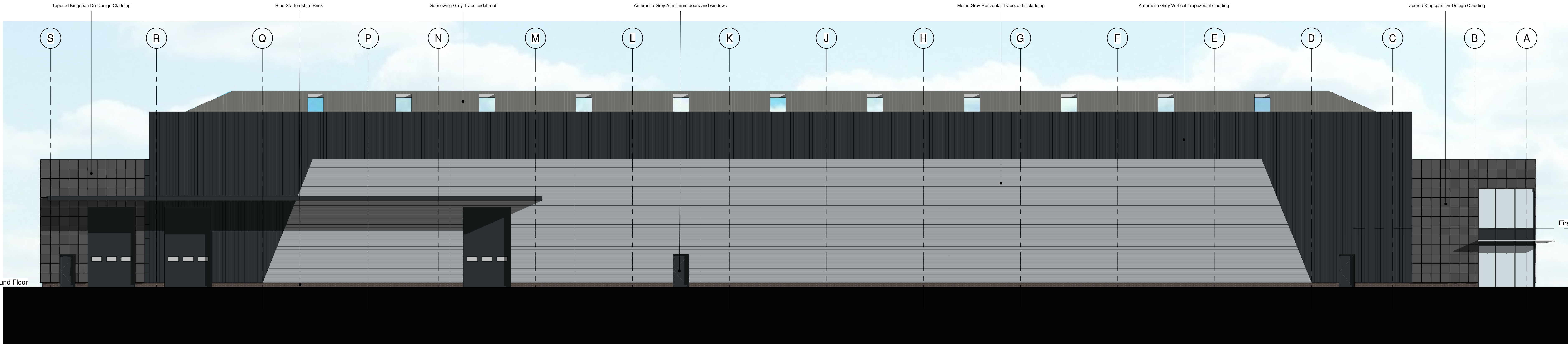
East Elevation 1 : 100
