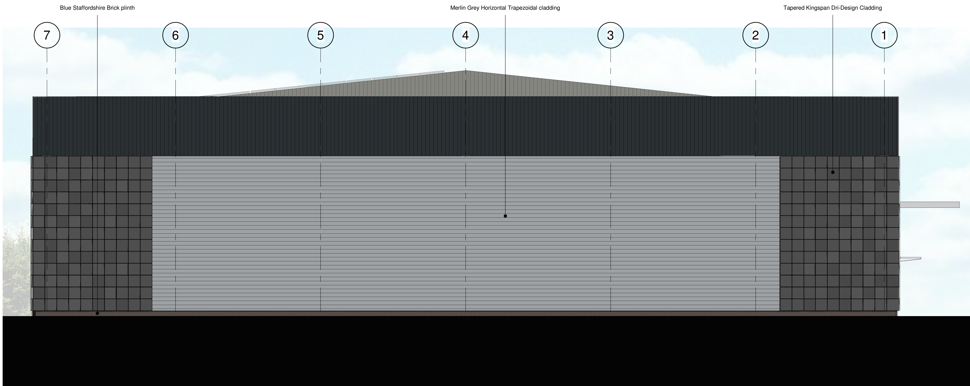
South Elevation 1 : 100
