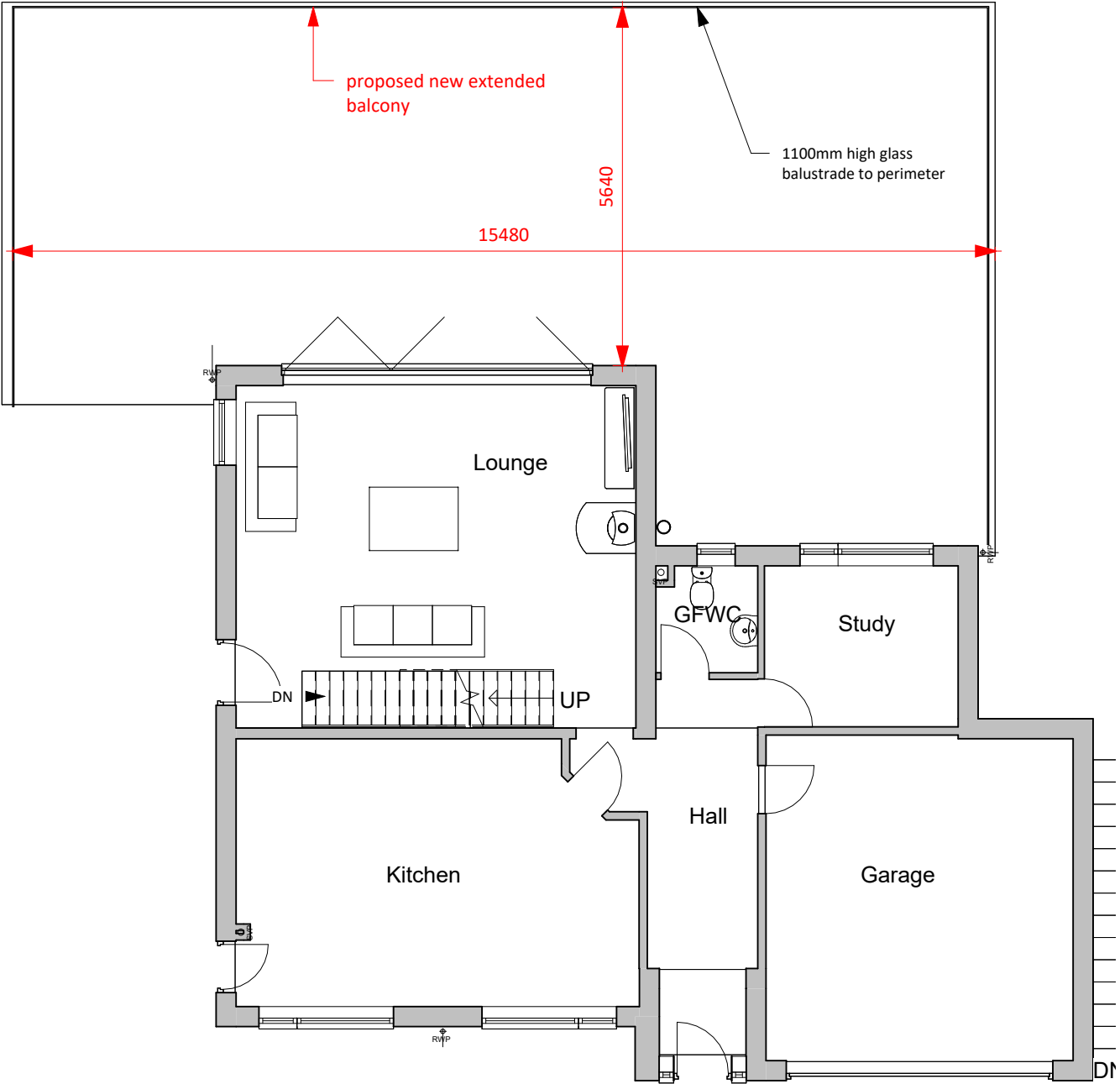
1 02b GF Proposed 1 : 100
