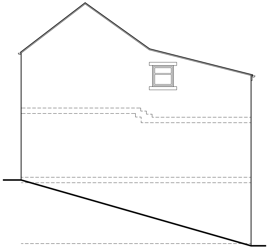
WEST ELEVATION
