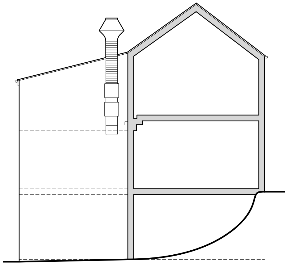
EAST ELEVATION
