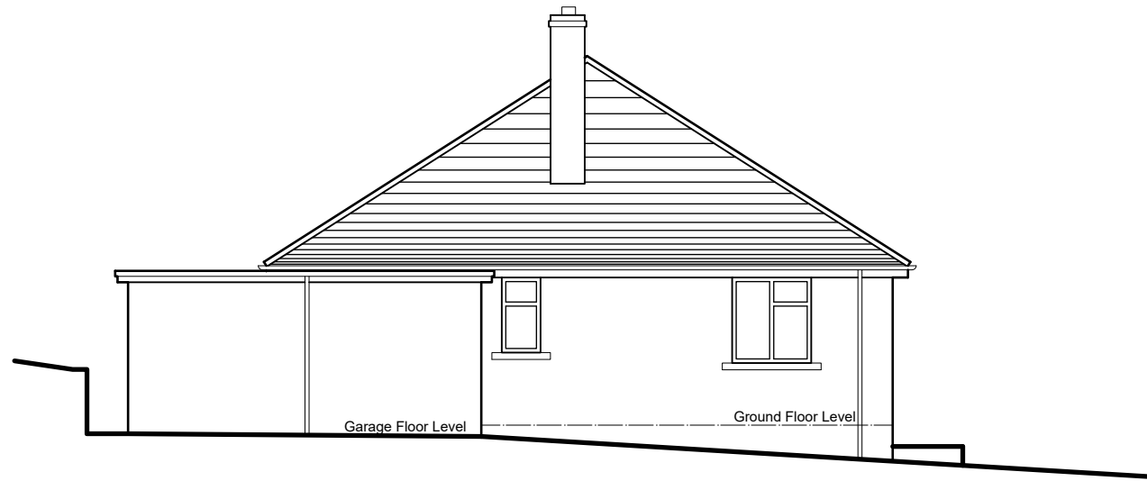
South West Elevation (side)
