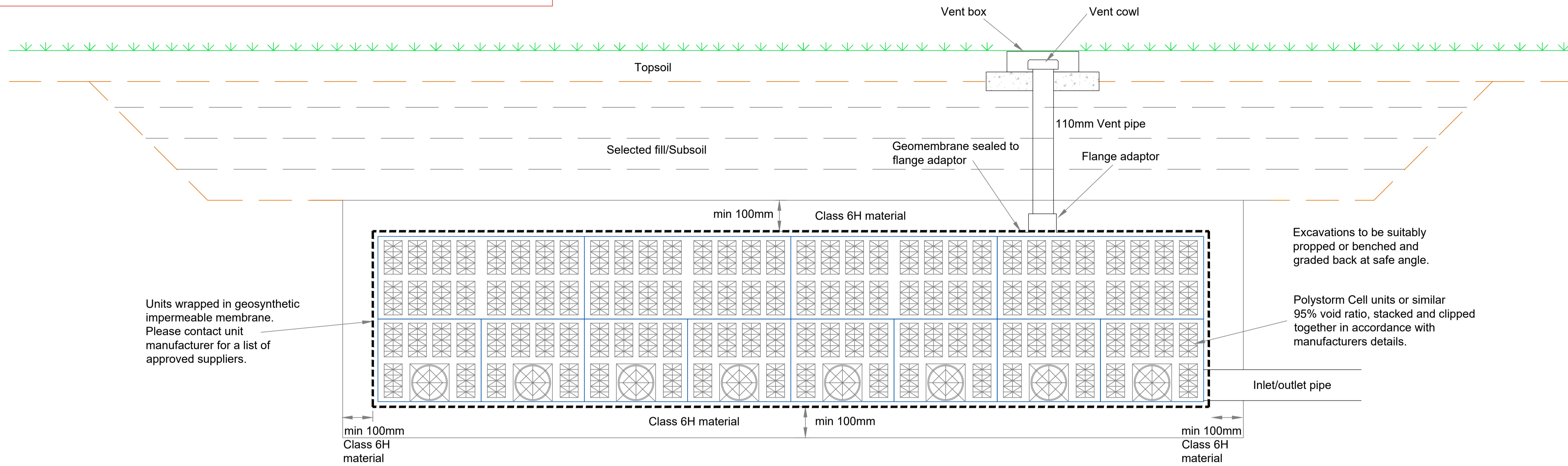
Typical Offline Cell Unit Attenuation tank
