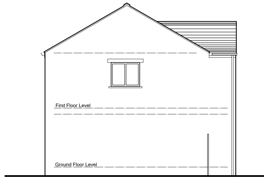
North West Elevation (side)
