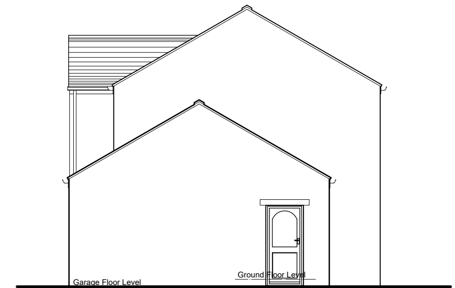
South East Elevation (side)
