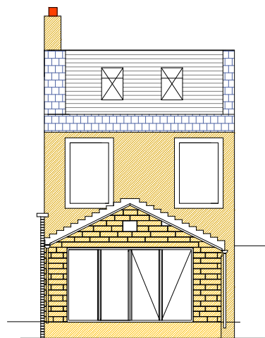
North Elevation/Rear
