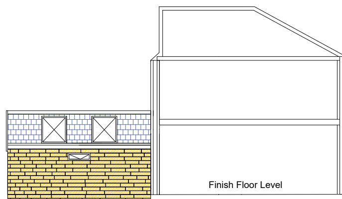
West Elevation
