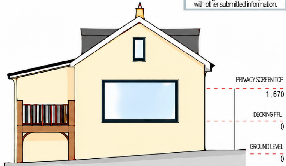
EAST ELEVATION
