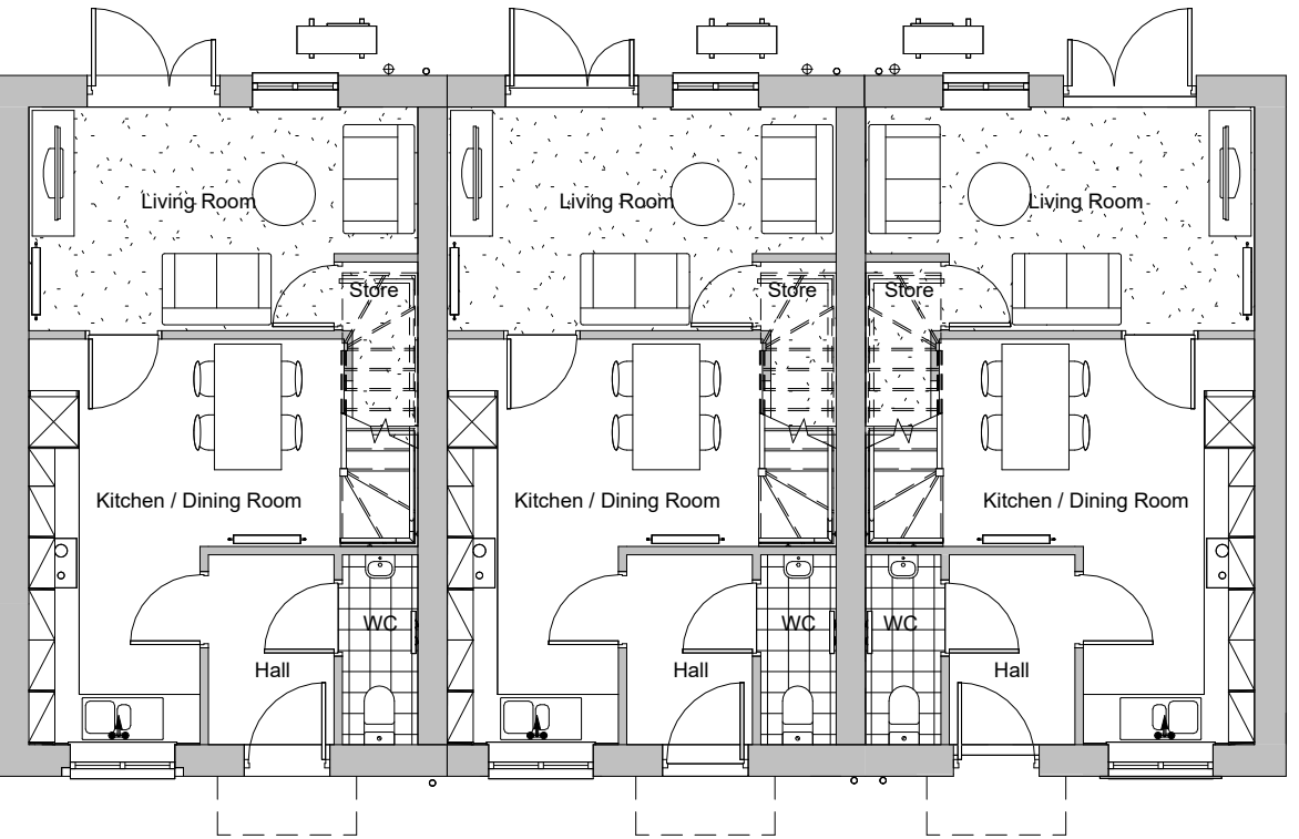
Plots 12-14 Ground Floor 1 : 100
