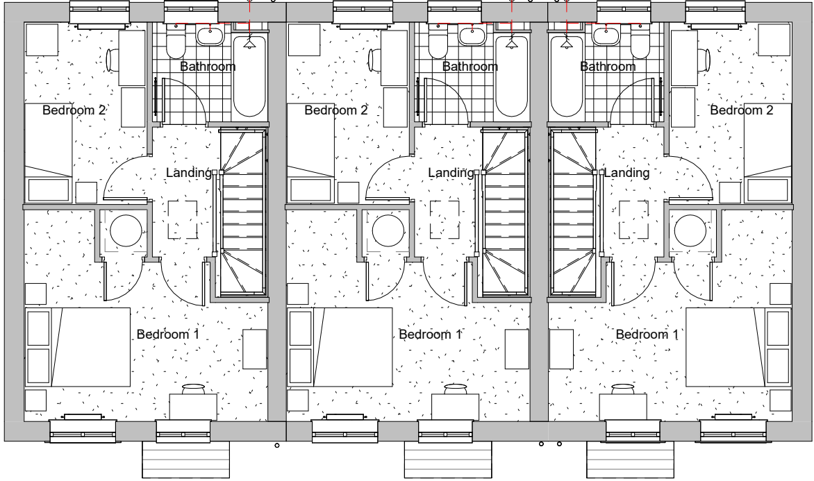
Plots 12-14 First Floor 1 : 100
