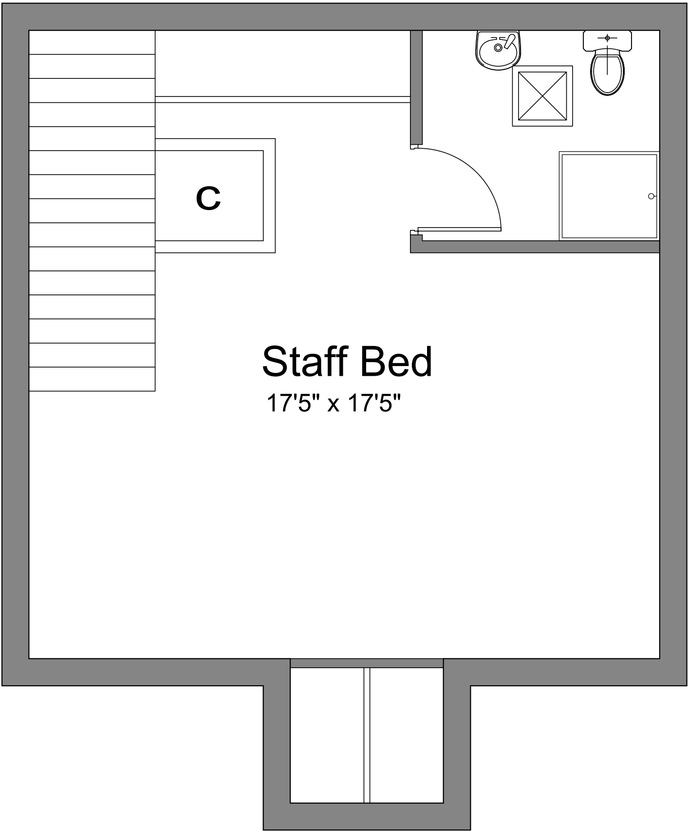
2nd Floor
