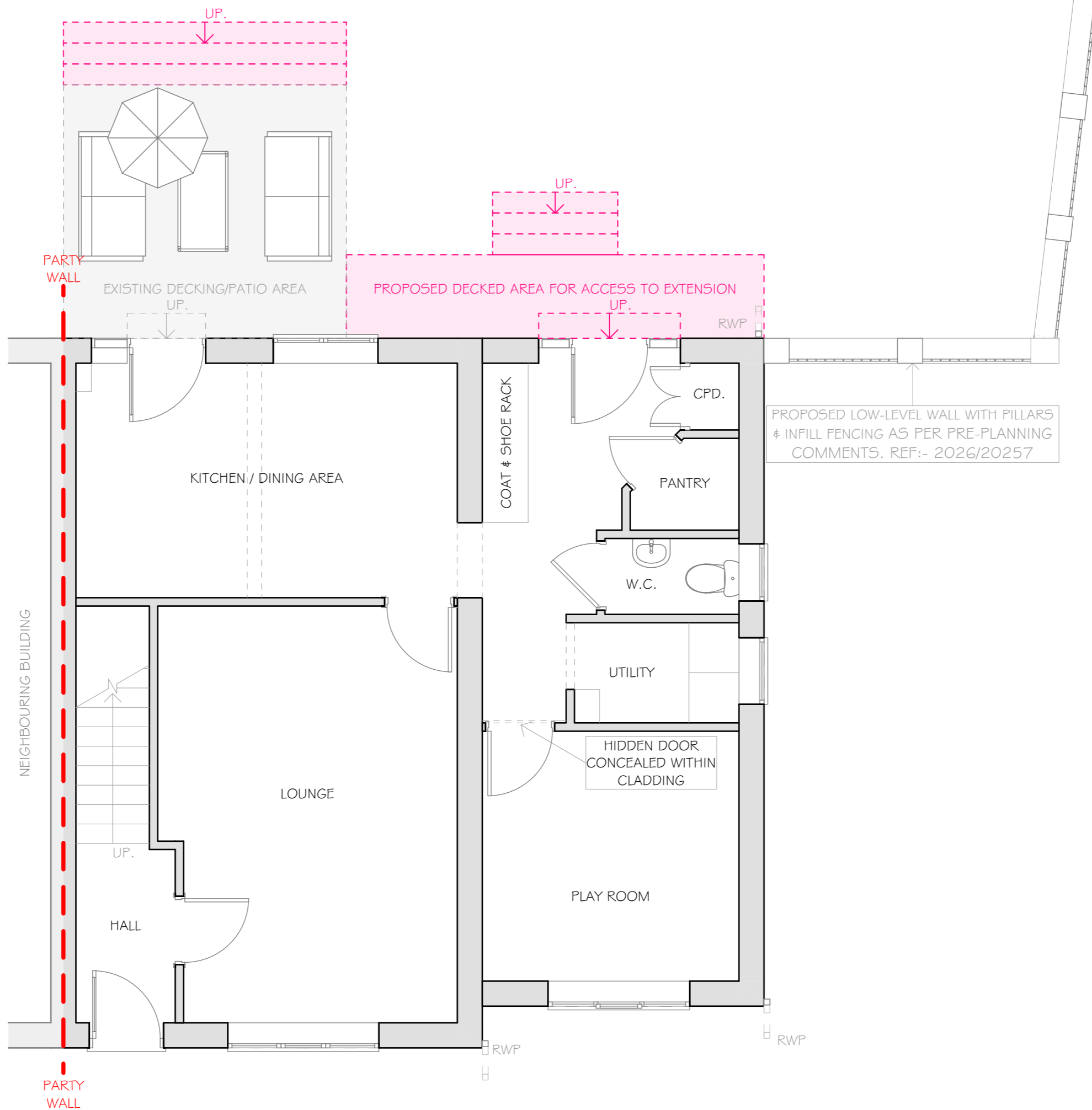
PROPOSED GROUND FLOOR PLAN 1:50@A3
