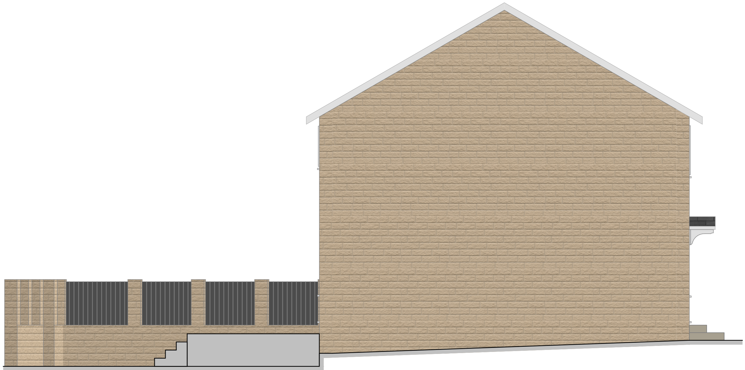
PROPOSED SIDE 2 ELEVATION 1:50@A3
