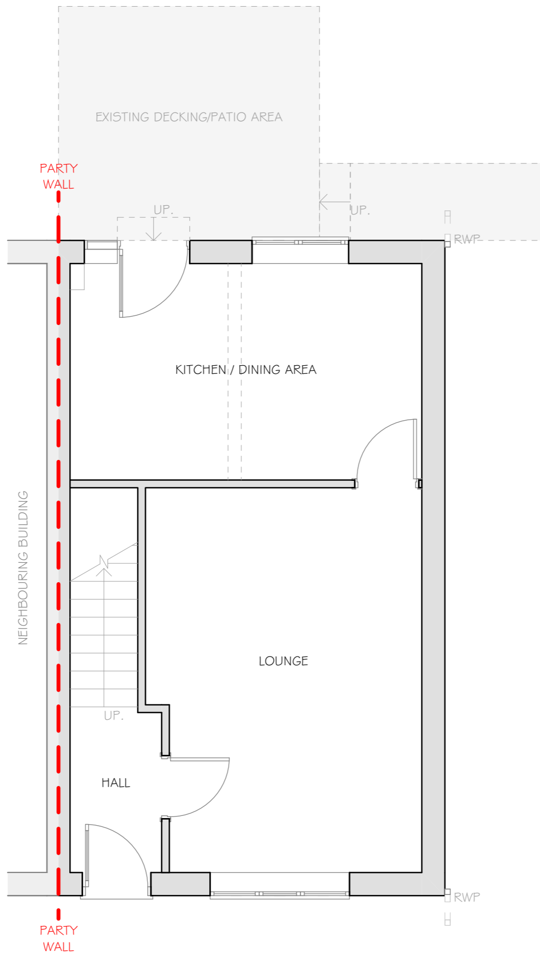
EXISTING GROUND FLOOR PLAN 1:50@A3
