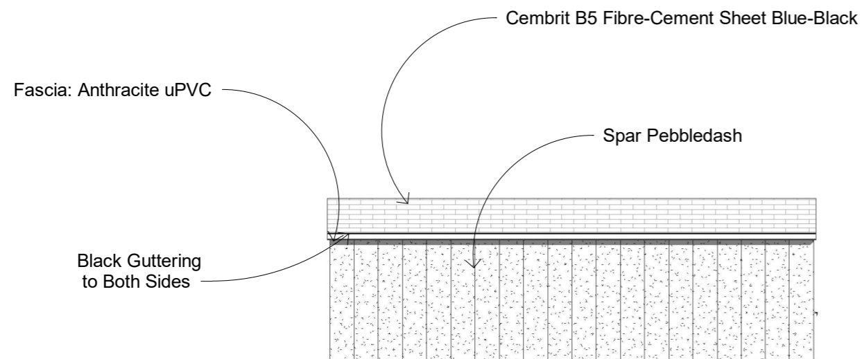
1 Rear Elevation 1 : 100
