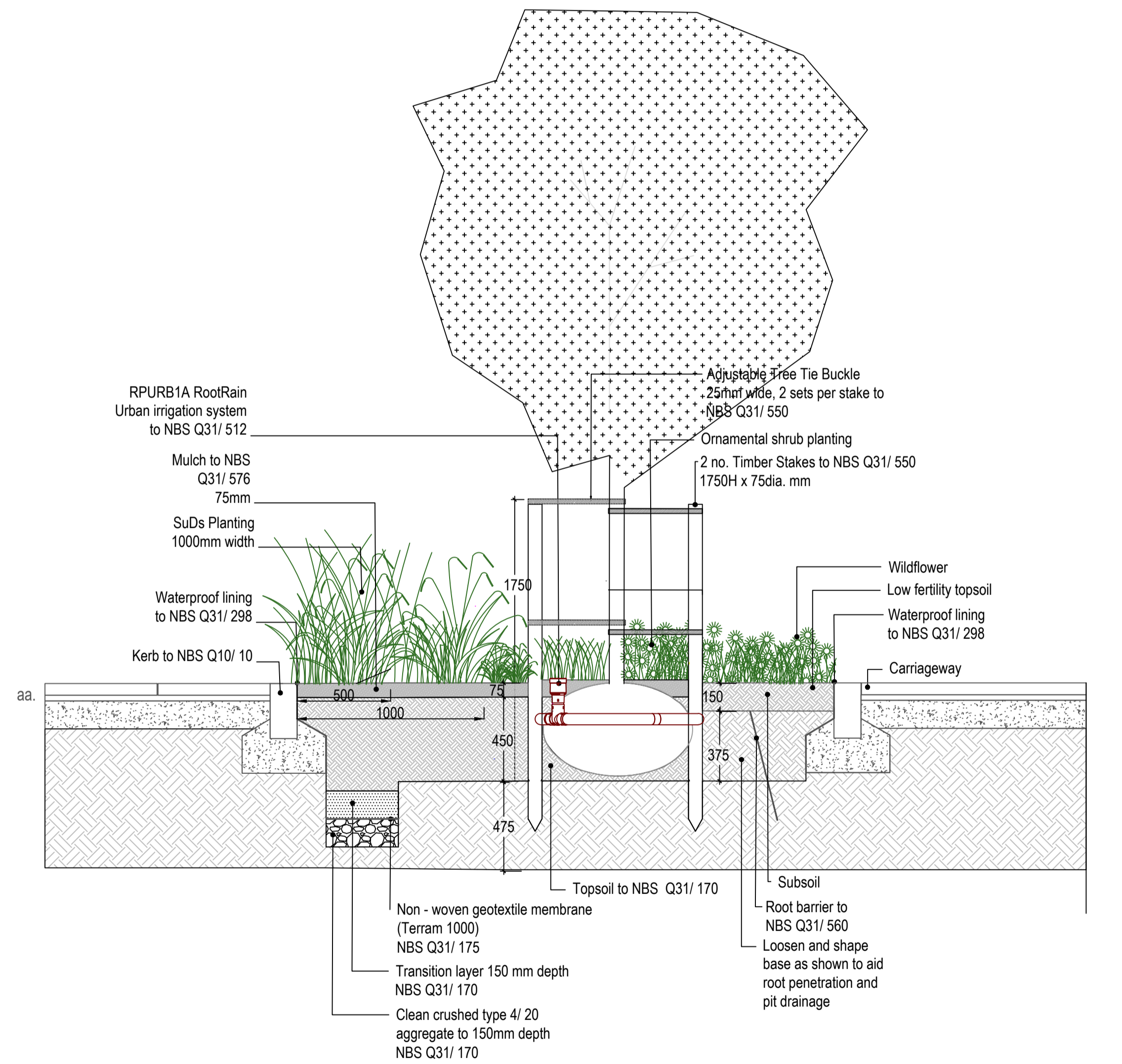
a Section a - Section through raised planting to north of site 1: 20 @A1
