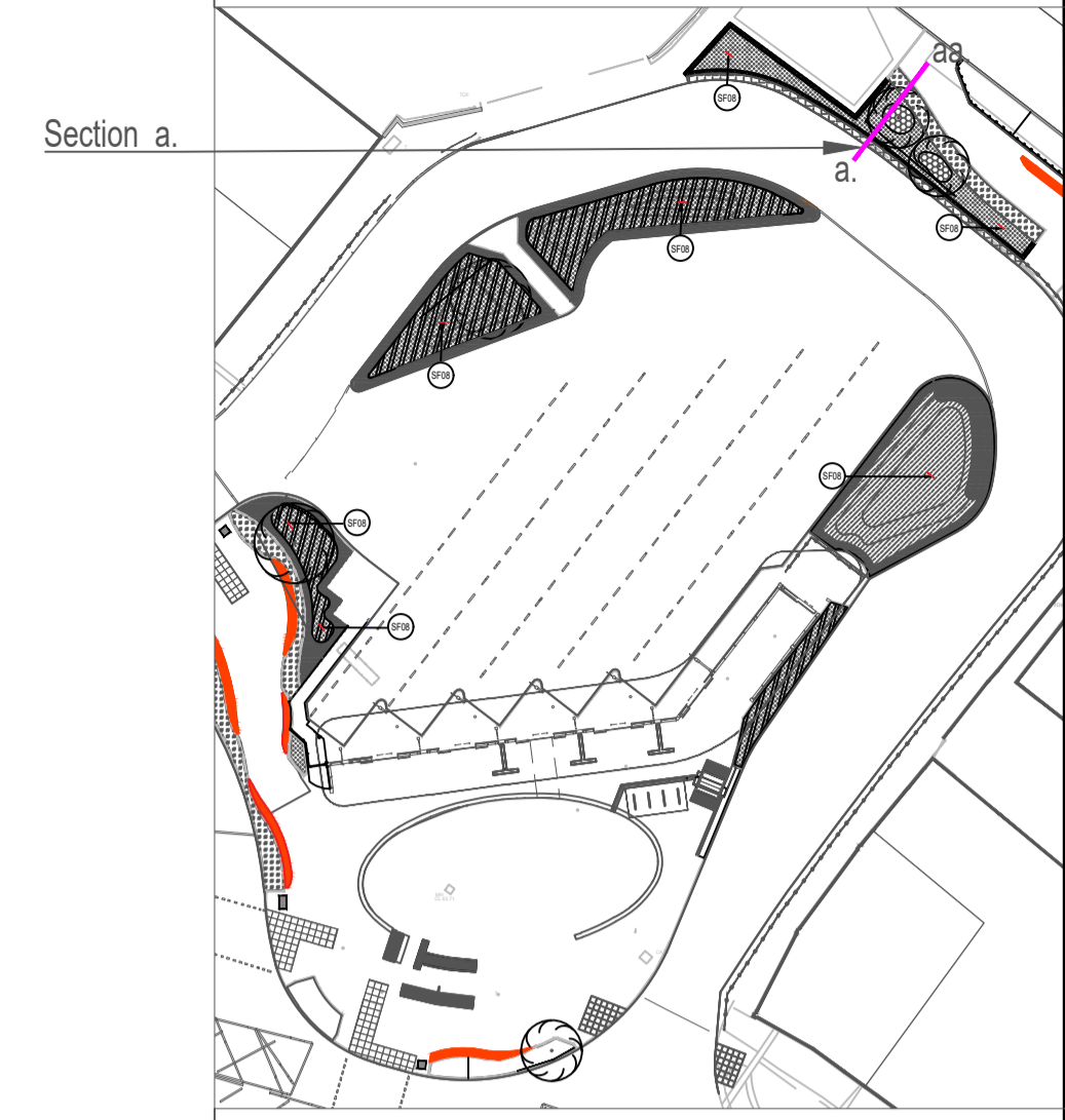
Section a. Location Plan
