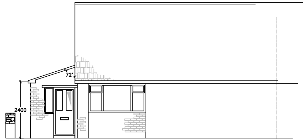
Elevation Front
