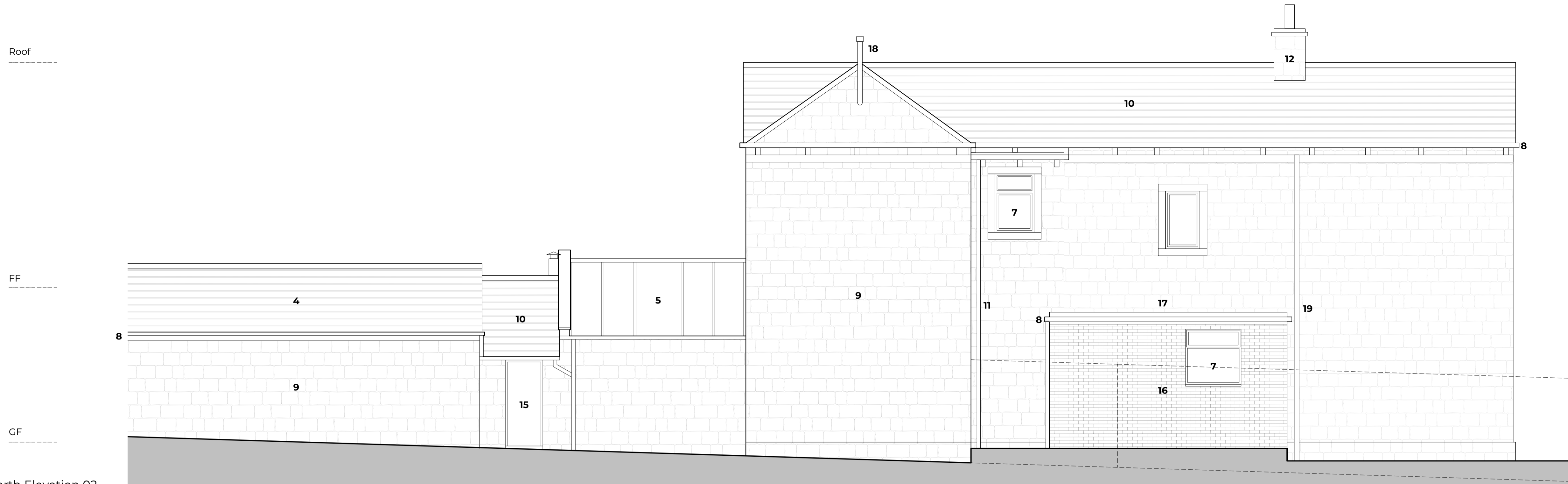
EX Existing North Elevation 02
