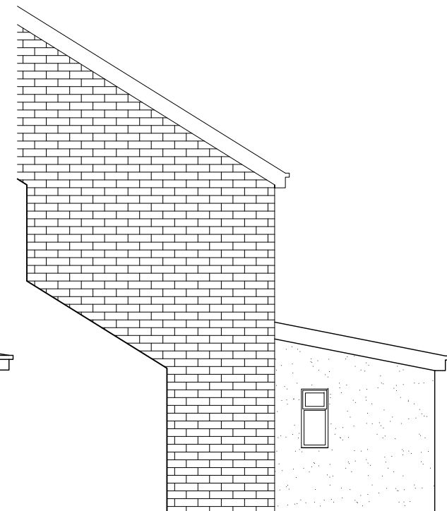
PROPOSED OTHER SIDE ELEVATION
