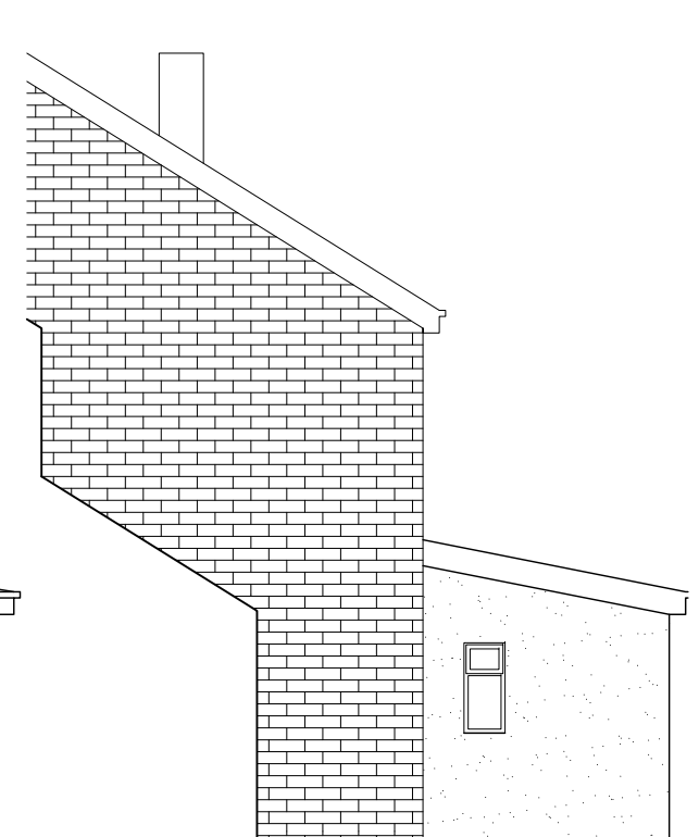
EXISTING AND PROPOSED OTHER SIDE ELEVATION
