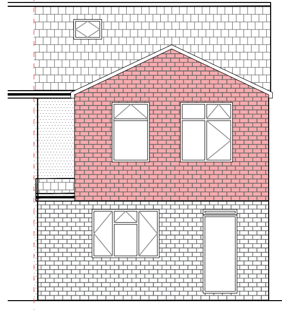
PROPOSED REAR ELEVATION (West)
