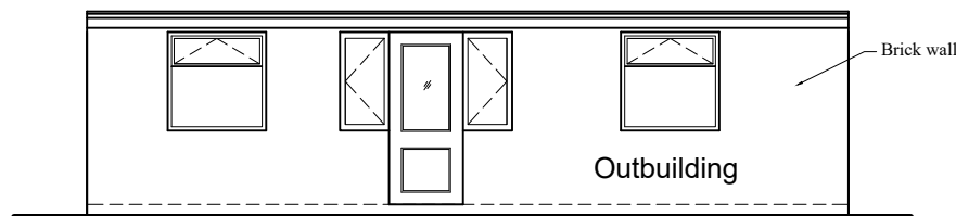
FRONT ELEVATION
