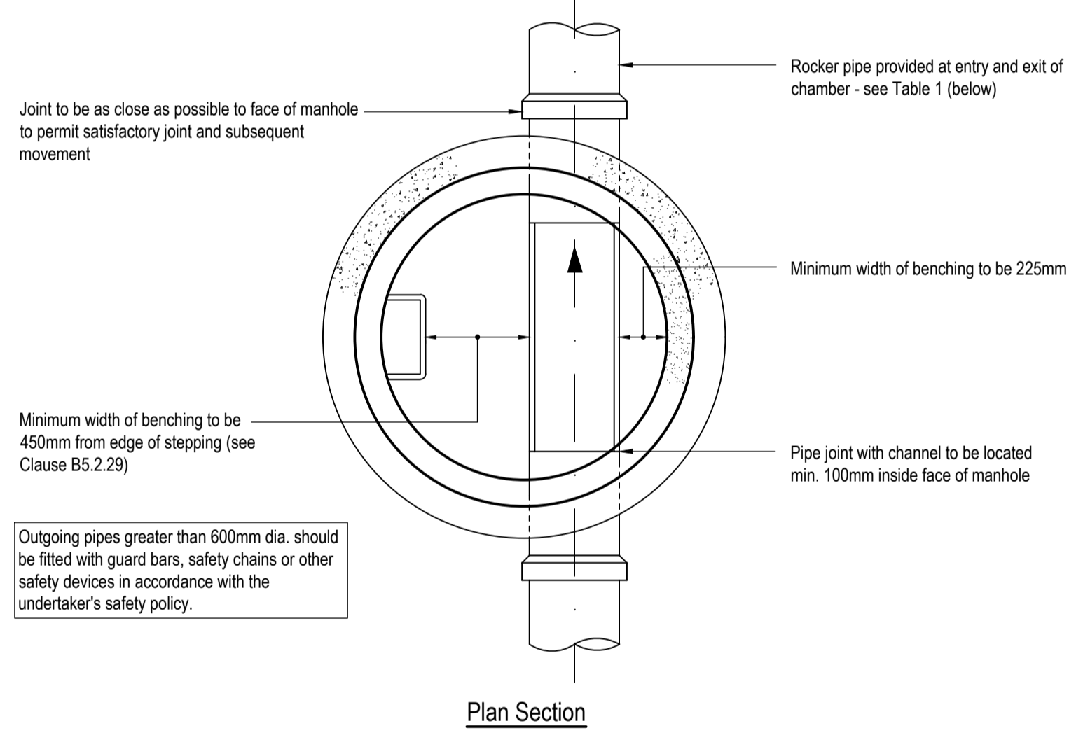
Typical Manhole Detail - Type C Depth from ground level to soffit of pipe 1.0m - 1.5m (Scale: 1:25)
