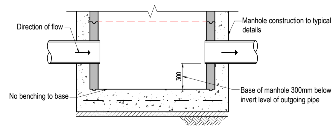
Typical Catchpit Manhole Detail - Type B Scale: 1:25
