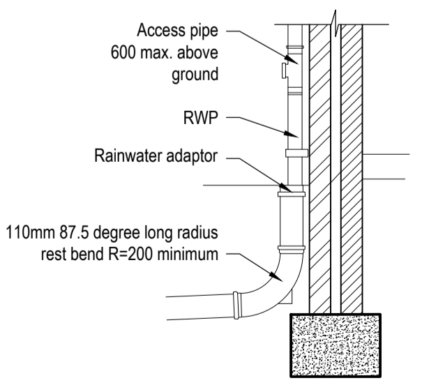
External RWP to Drain
