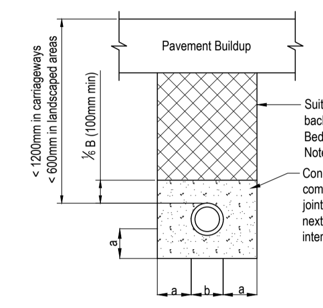
Drainage Shallow Pipe Bedding Detail
