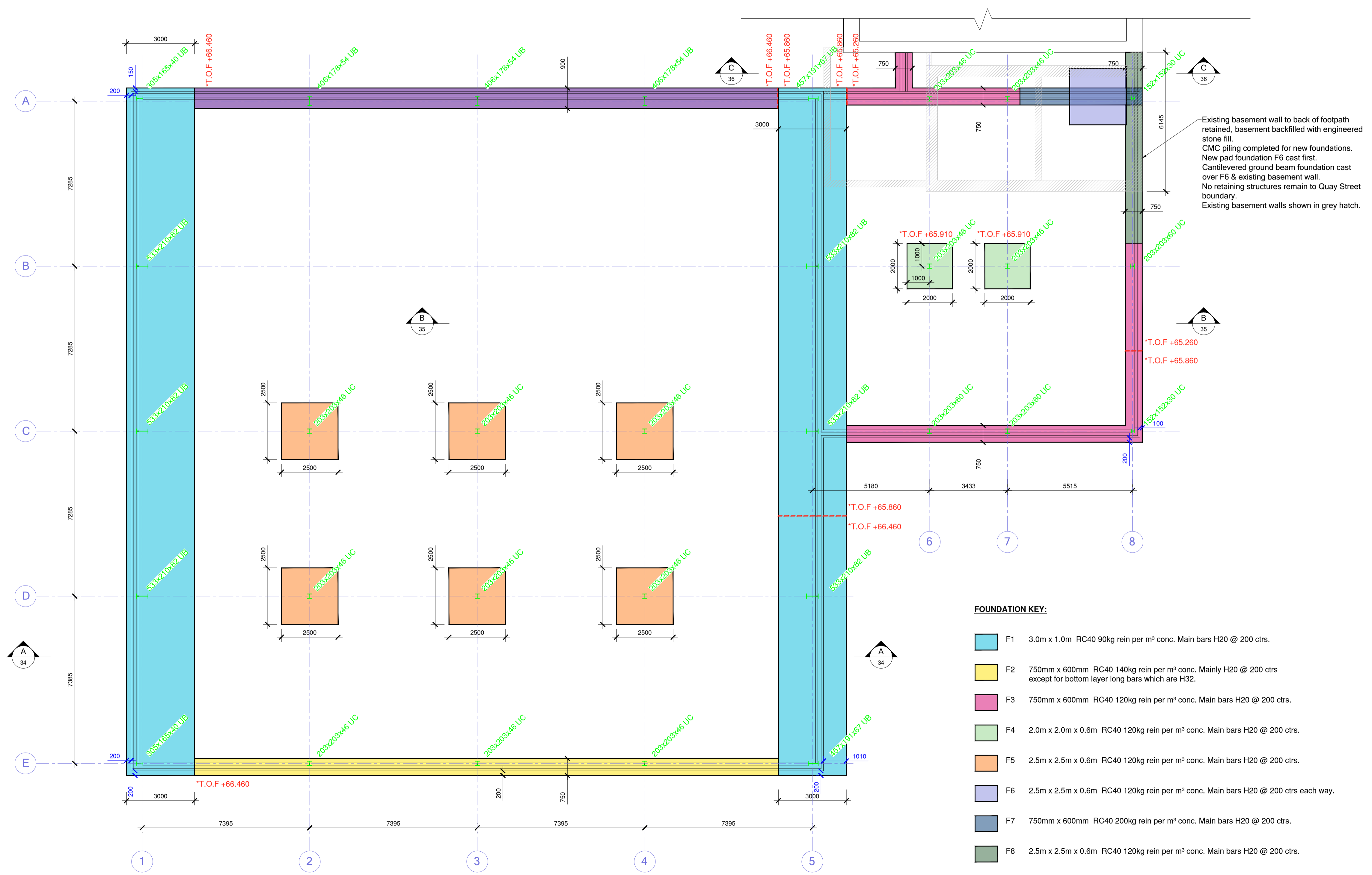
PROPOSED SUB-STRUCTURE PLAN SCALE: 1:100
