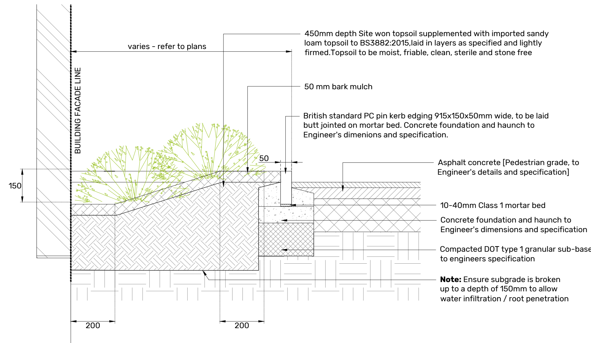
Planting to building interface - Typical Detail Scale 1:10
