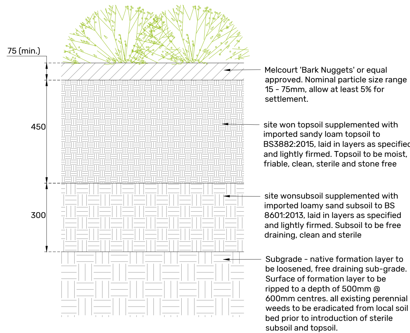
Ornamental Planting - Typical Detail Scale 1:10
