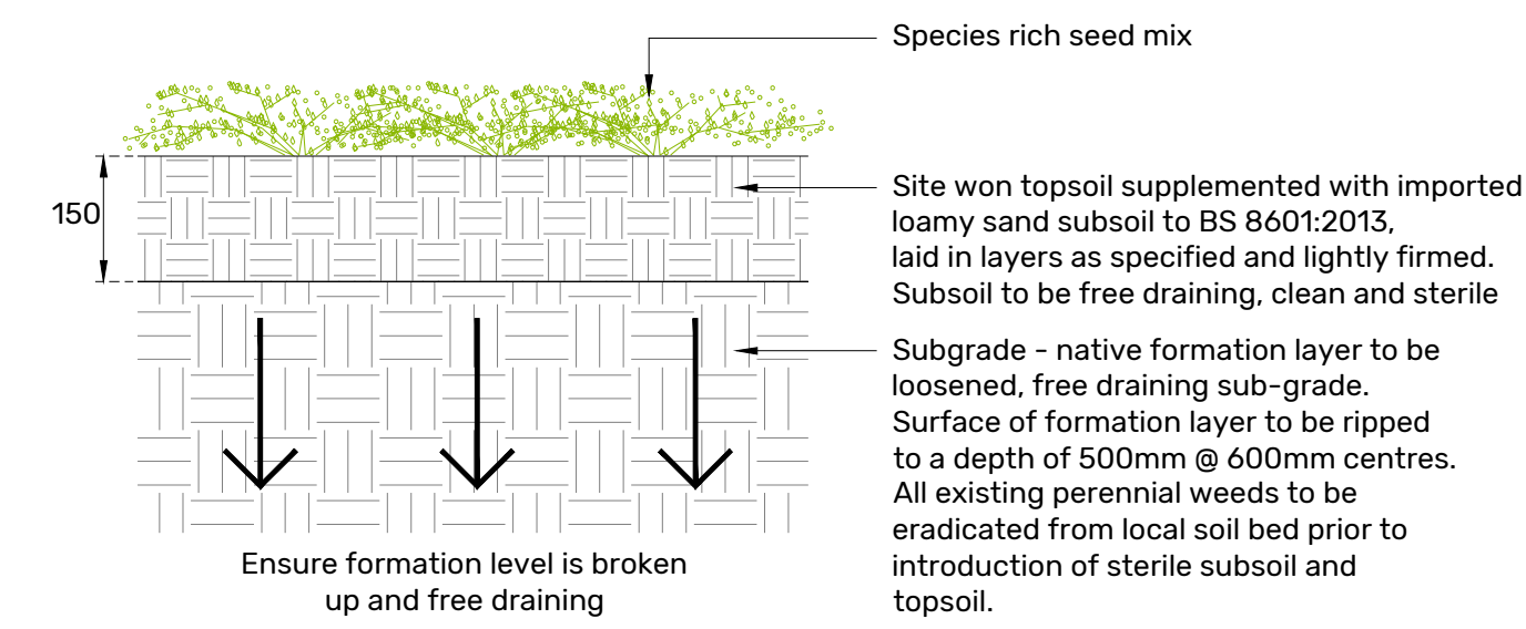
Species Rich Grass Seeding - Typical Detail Scale 1:10
