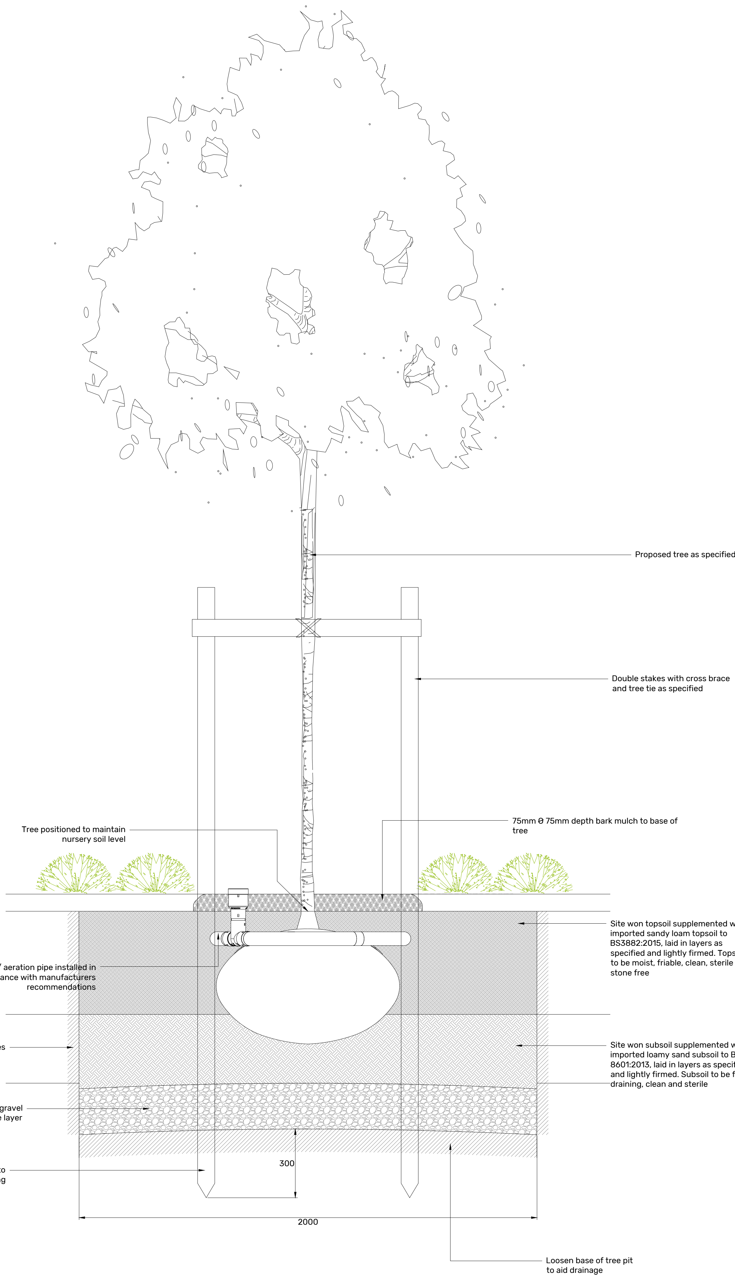
Tree Pit - Typical Detail Scale 1:10
