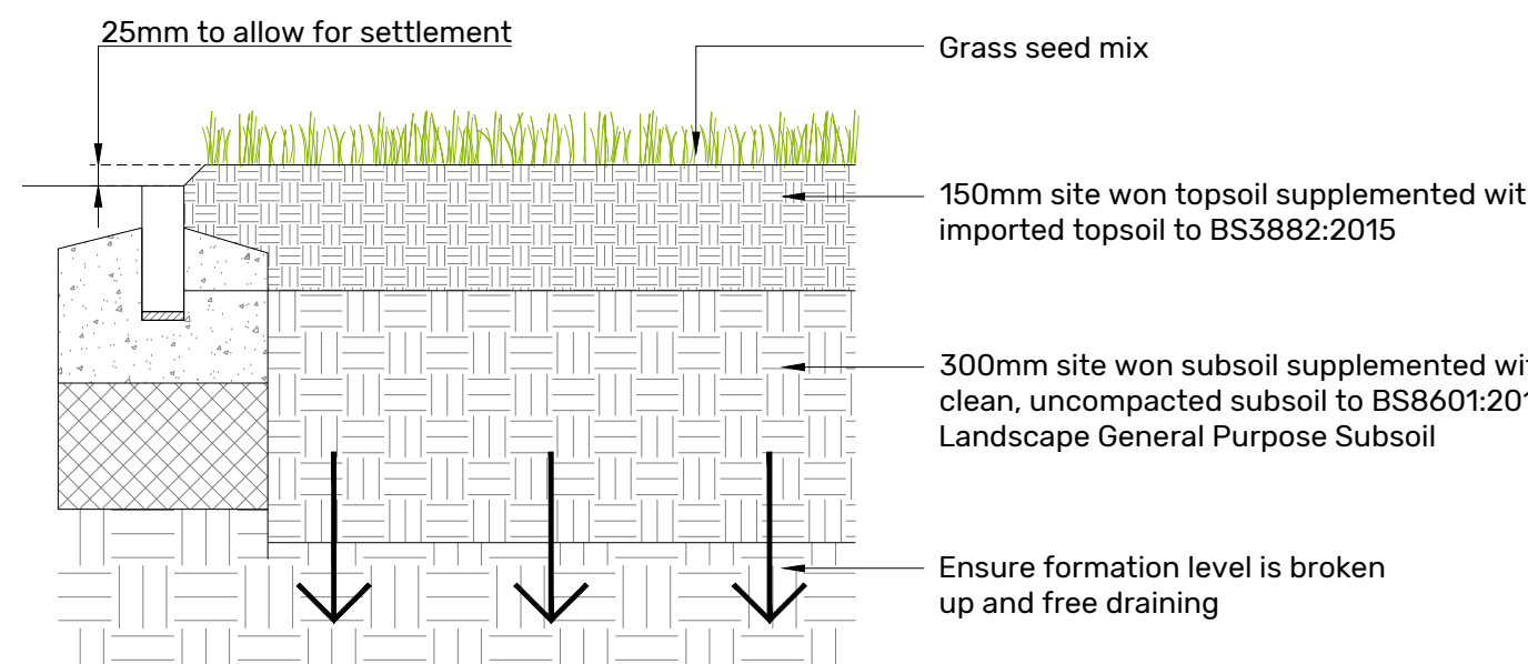
Grass Seeding - Typical Detail Scale 1:10
