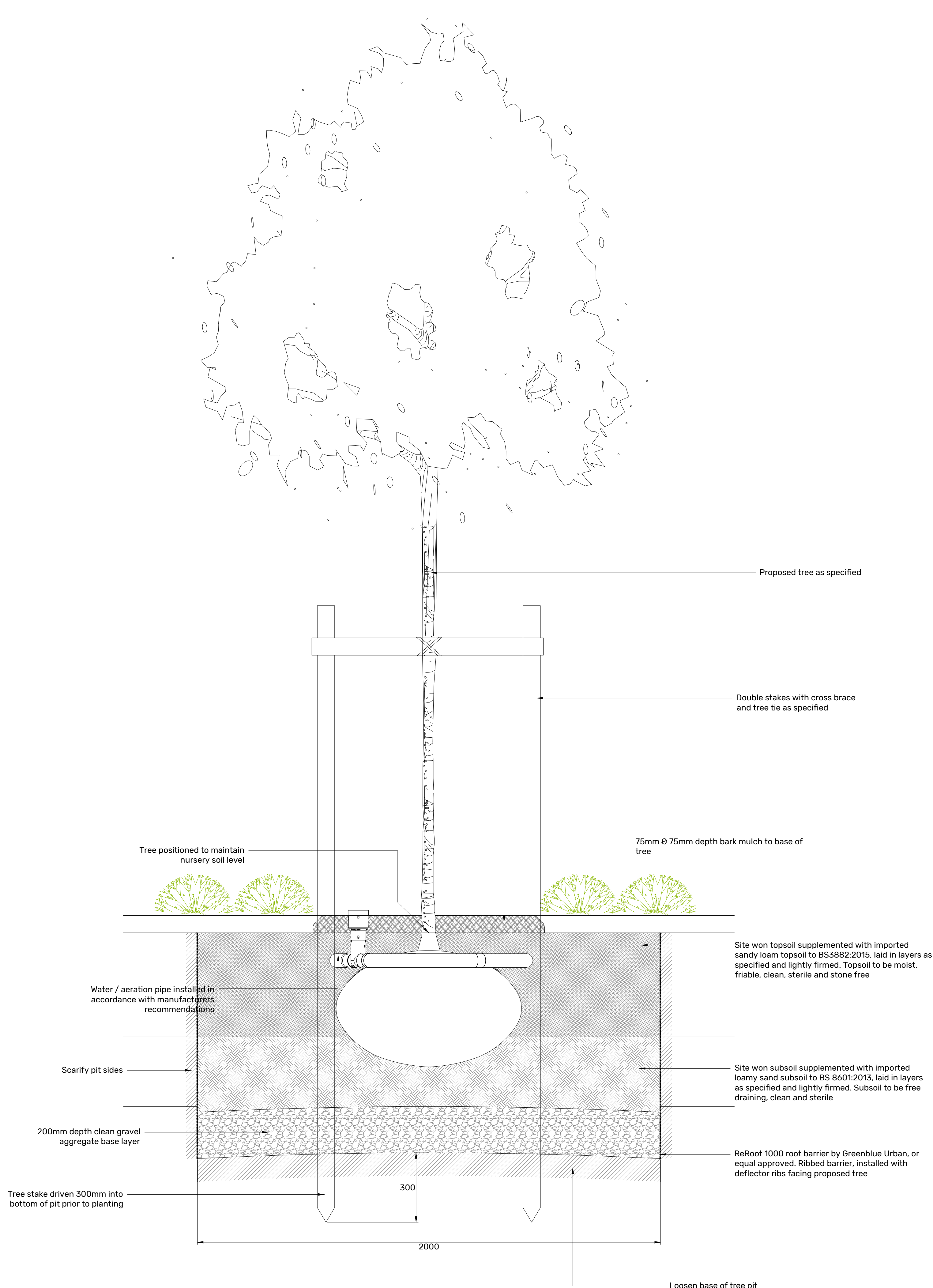
Root Barrier Tree Pit - Typical Scale 1:10
