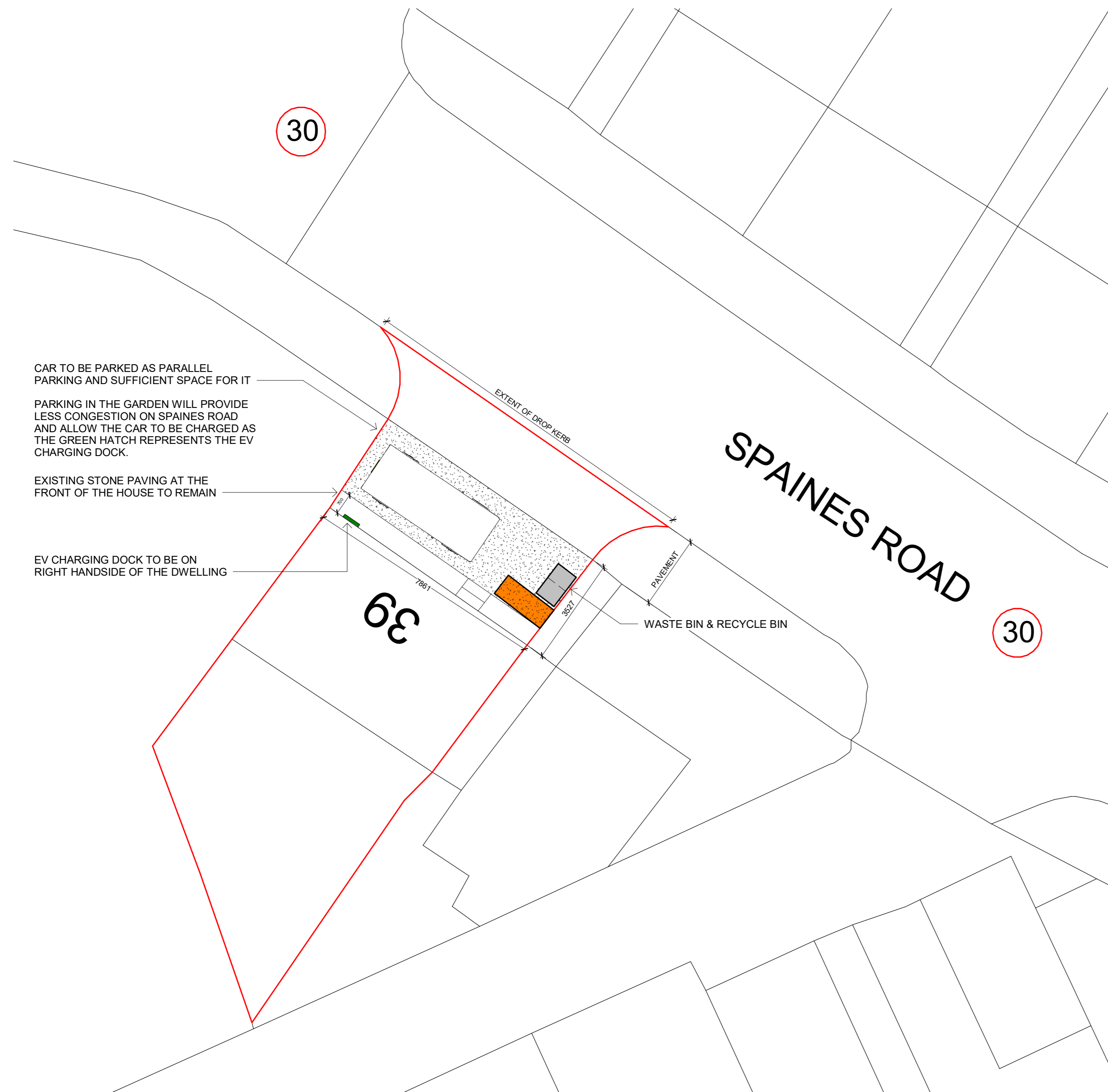
1 Proposed Plan - with car on plan 1 : 100
