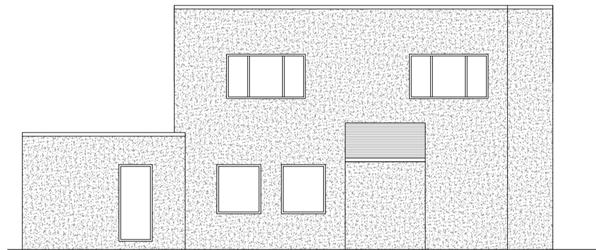
North Elevation 1.100
