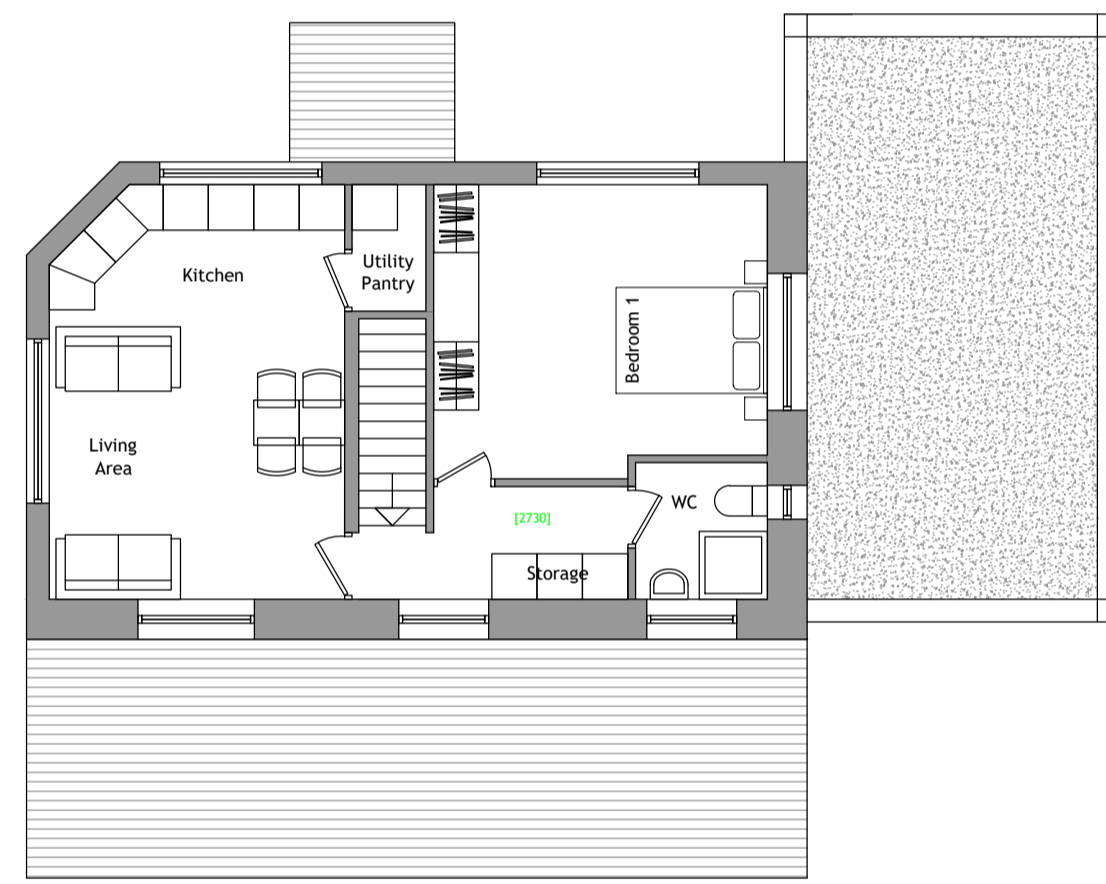
First Floor Layout 1.100
