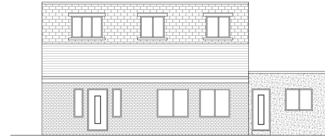
South Elevation 1.100
