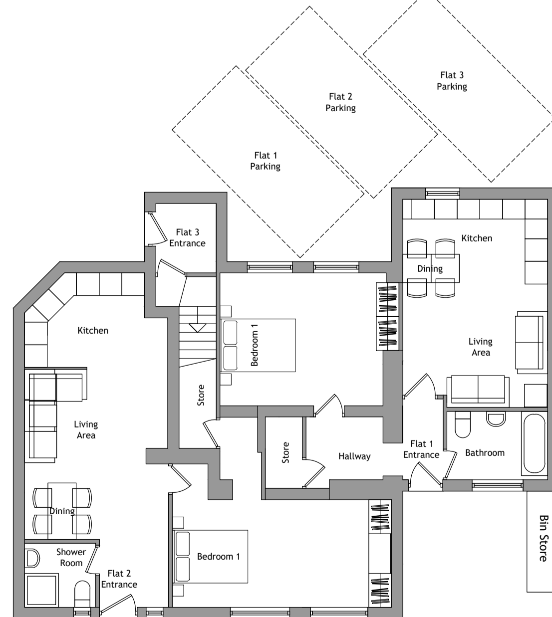
Ground Floor Layout 1.100
