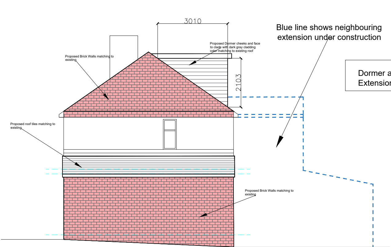
PROPOSED SIDE ELEVATION (North West)
